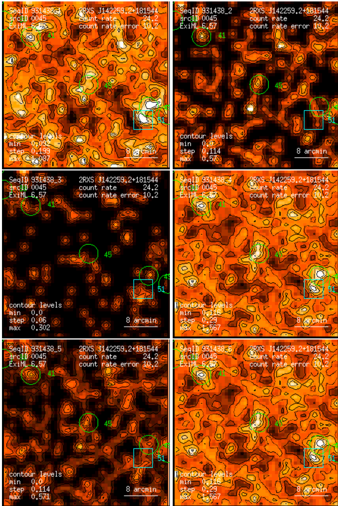
Figure 45: RASS 931438: detection 0045: band rate images, Gaussian filter: (1) PSPC channels 11 – 41, (2) 52 – 90, (3) 91 – 201, (4) 11 – 235, (5) 52 – 201, (6) 11 – 201. Broad band rates in counts/ks. Band rate contour levels in counts/ks/arcmin 2 .
