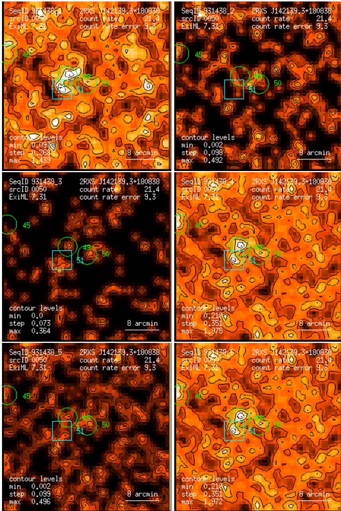
Figure 50: RASS 931438: detection 0050: band rate images, Gaussian filter: (1) PSPC channels 11 – 41, (2) 52 – 90, (3) 91 – 201, (4) 11 – 235, (5) 52 – 201, (6) 11 – 201. Broad band rates in counts/ks. Band rate contour levels in counts/ks/arcmin 2 .
