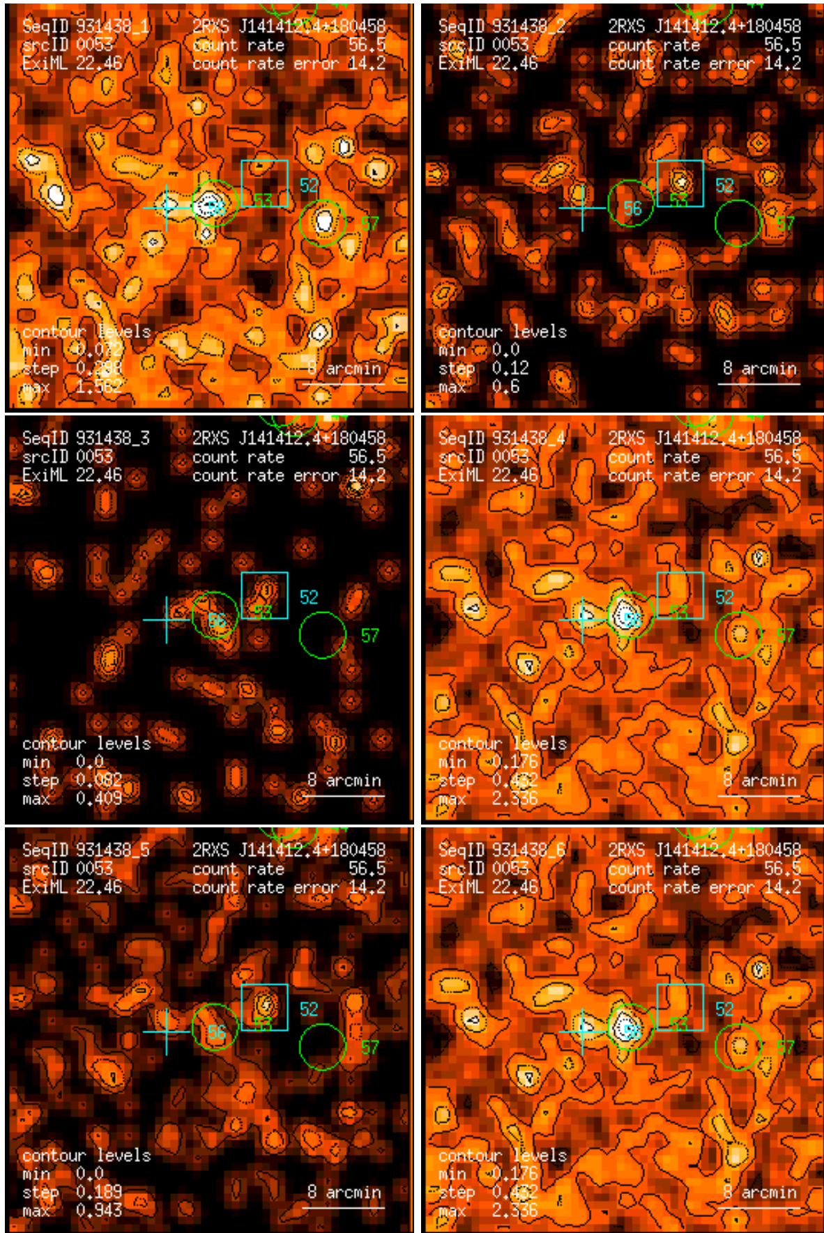
Figure 53: RASS 931438: detection 0053: band rate images, Gaussian filter: (1) PSPC channels 11 – 41, (2) 52 – 90, (3) 91 – 201, (4) 11 – 235, (5) 52 – 201, (6) 11 – 201. Broad band rates in counts/ks. Band rate contour levels in counts/ks/arcmin 2 .
