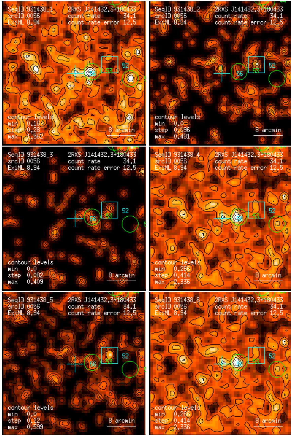
Figure 56: RASS 931438: detection 0056: band rate images, Gaussian filter: (1) PSPC channels 11 – 41, (2) 52 – 90, (3) 91 – 201, (4) 11 – 235, (5) 52 – 201, (6) 11 – 201. Broad band rates in counts/ks. Band rate contour levels in counts/ks/arcmin 2 .
