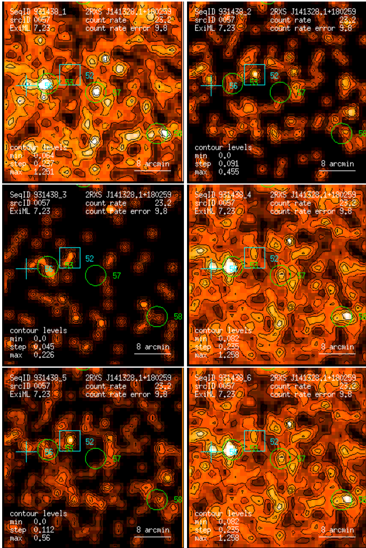
Figure 57: RASS 931438: detection 0057: band rate images, Gaussian filter: (1) PSPC channels 11 – 41, (2) 52 – 90, (3) 91 – 201, (4) 11 – 235, (5) 52 – 201, (6) 11 – 201. Broad band rates in counts/ks. Band rate contour levels in counts/ks/arcmin 2 .
