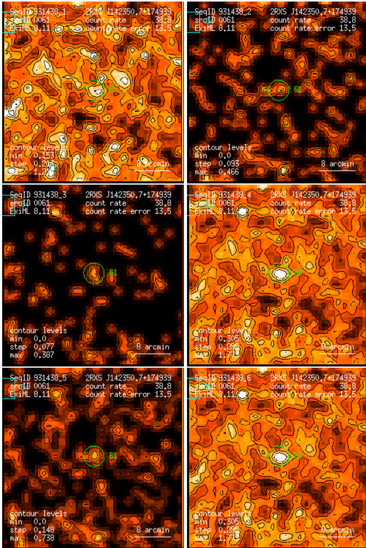
Figure 61: RASS 931438: detection 0061: band rate images, Gaussian filter: (1) PSPC channels 11 – 41, (2) 52 – 90, (3) 91 – 201, (4) 11 – 235, (5) 52 – 201, (6) 11 – 201. Broad band rates in counts/ks. Band rate contour levels in counts/ks/arcmin 2 .
