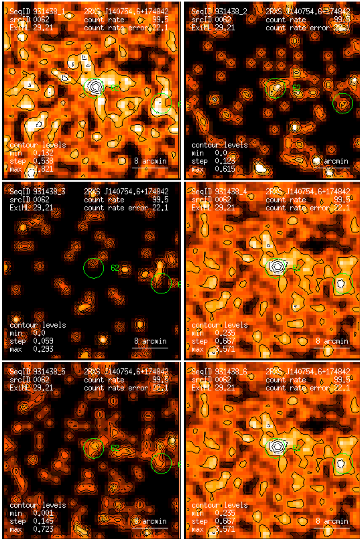
Figure 62: RASS 931438: detection 0062: band rate images, Gaussian filter: (1) PSPC channels 11 – 41, (2) 52 – 90, (3) 91 – 201, (4) 11 – 235, (5) 52 – 201, (6) 11 – 201. Broad band rates in counts/ks. Band rate contour levels in counts/ks/arcmin 2 .
