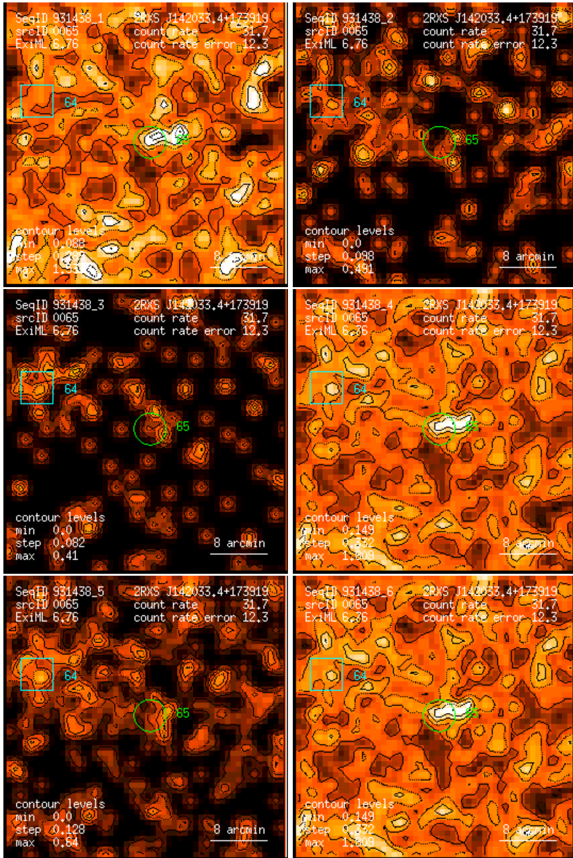
Figure 65: RASS 931438: detection 0065: band rate images, Gaussian filter: (1) PSPC channels 11 – 41, (2) 52 – 90, (3) 91 – 201, (4) 11 – 235, (5) 52 – 201, (6) 11 – 201. Broad band rates in counts/ks. Band rate contour levels in counts/ks/arcmin 2 .
