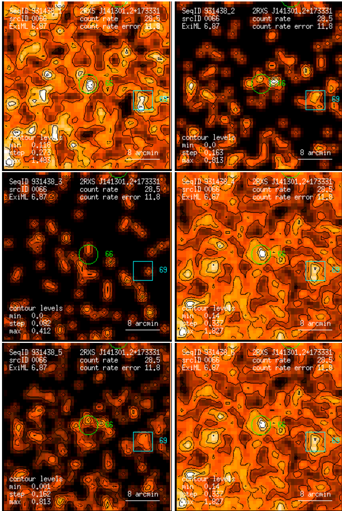
Figure 66: RASS 931438: detection 0066: band rate images, Gaussian filter: (1) PSPC channels 11 – 41, (2) 52 – 90, (3) 91 – 201, (4) 11 – 235, (5) 52 – 201, (6) 11 – 201. Broad band rates in counts/ks. Band rate contour levels in counts/ks/arcmin 2 .
