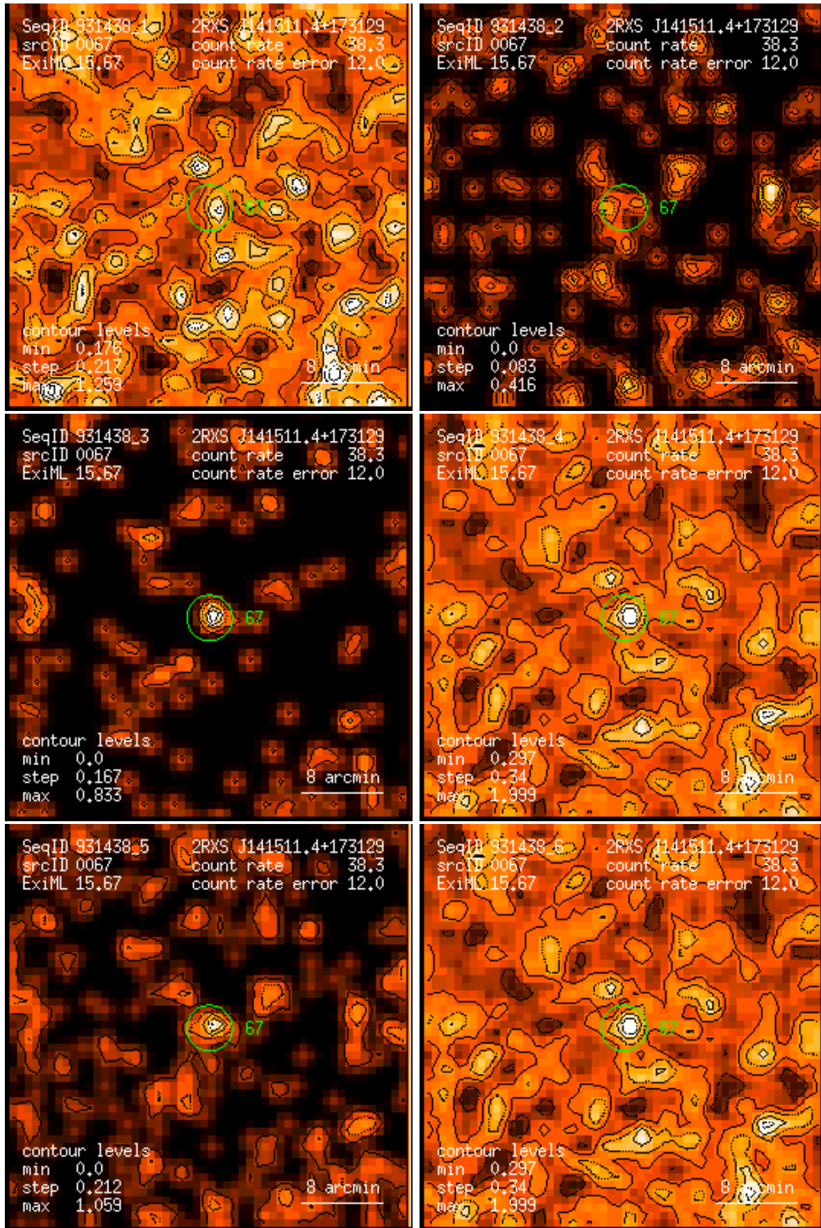
Figure 67: RASS 931438: detection 0067: band rate images, Gaussian filter: (1) PSPC channels 11 – 41, (2) 52 – 90, (3) 91 – 201, (4) 11 – 235, (5) 52 – 201, (6) 11 – 201. Broad band rates in counts/ks. Band rate contour levels in counts/ks/arcmin 2 .
