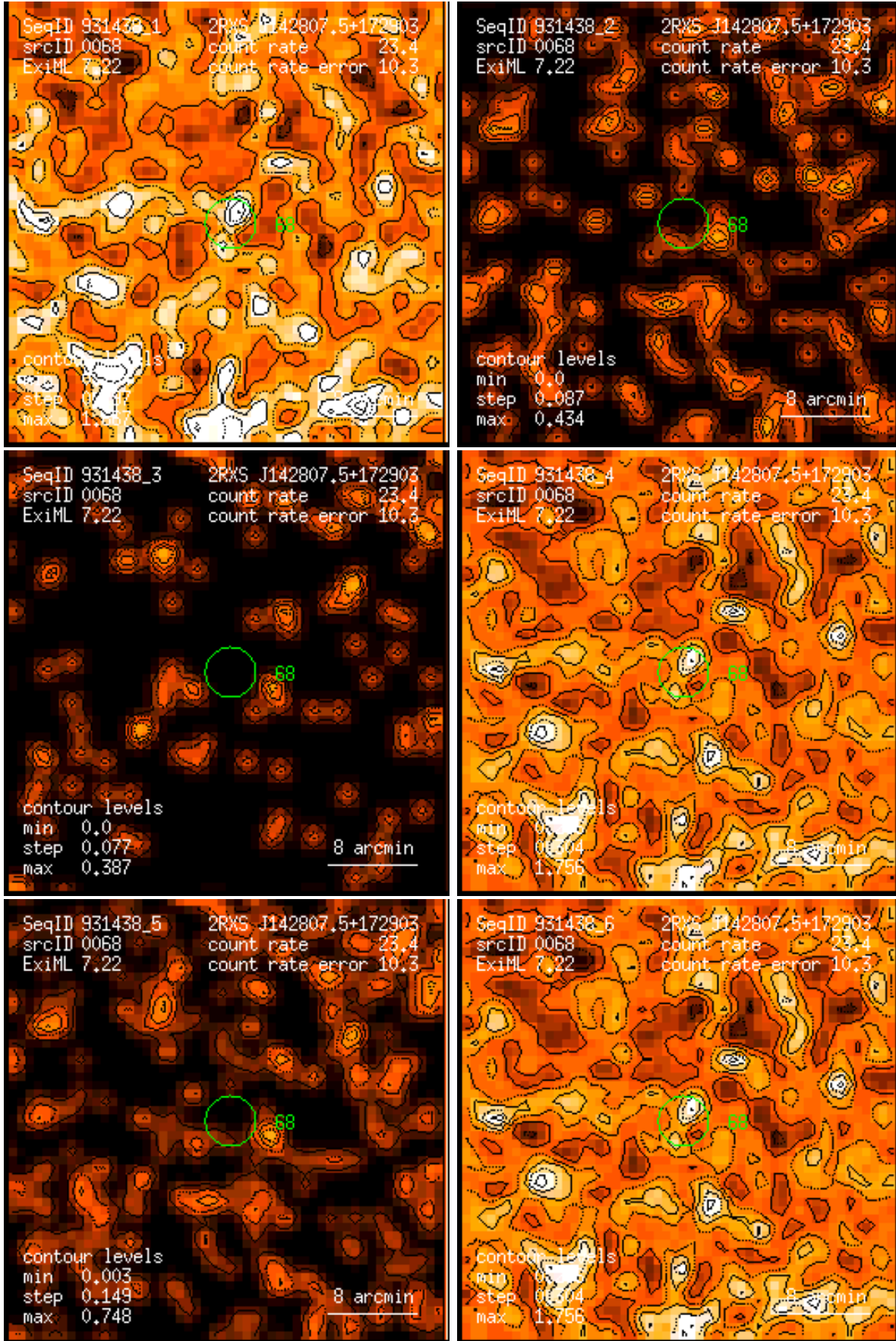
Figure 68: RASS 931438: detection 0068: band rate images, Gaussian filter: (1) PSPC channels 11 – 41, (2) 52 – 90, (3) 91 – 201, (4) 11 – 235, (5) 52 – 201, (6) 11 – 201. Broad band rates in counts/ks. Band rate contour levels in counts/ks/arcmin 2 .
