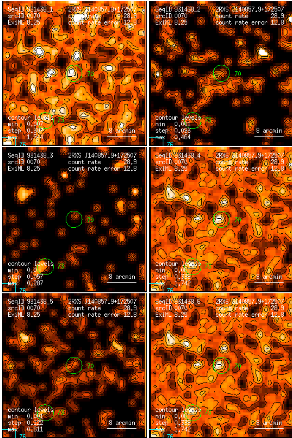
Figure 70: RASS 931438: detection 0070: band rate images, Gaussian filter: (1) PSPC channels 11 – 41, (2) 52 – 90, (3) 91 – 201, (4) 11 – 235, (5) 52 – 201, (6) 11 – 201. Broad band rates in counts/ks. Band rate contour levels in counts/ks/arcmin 2 .
