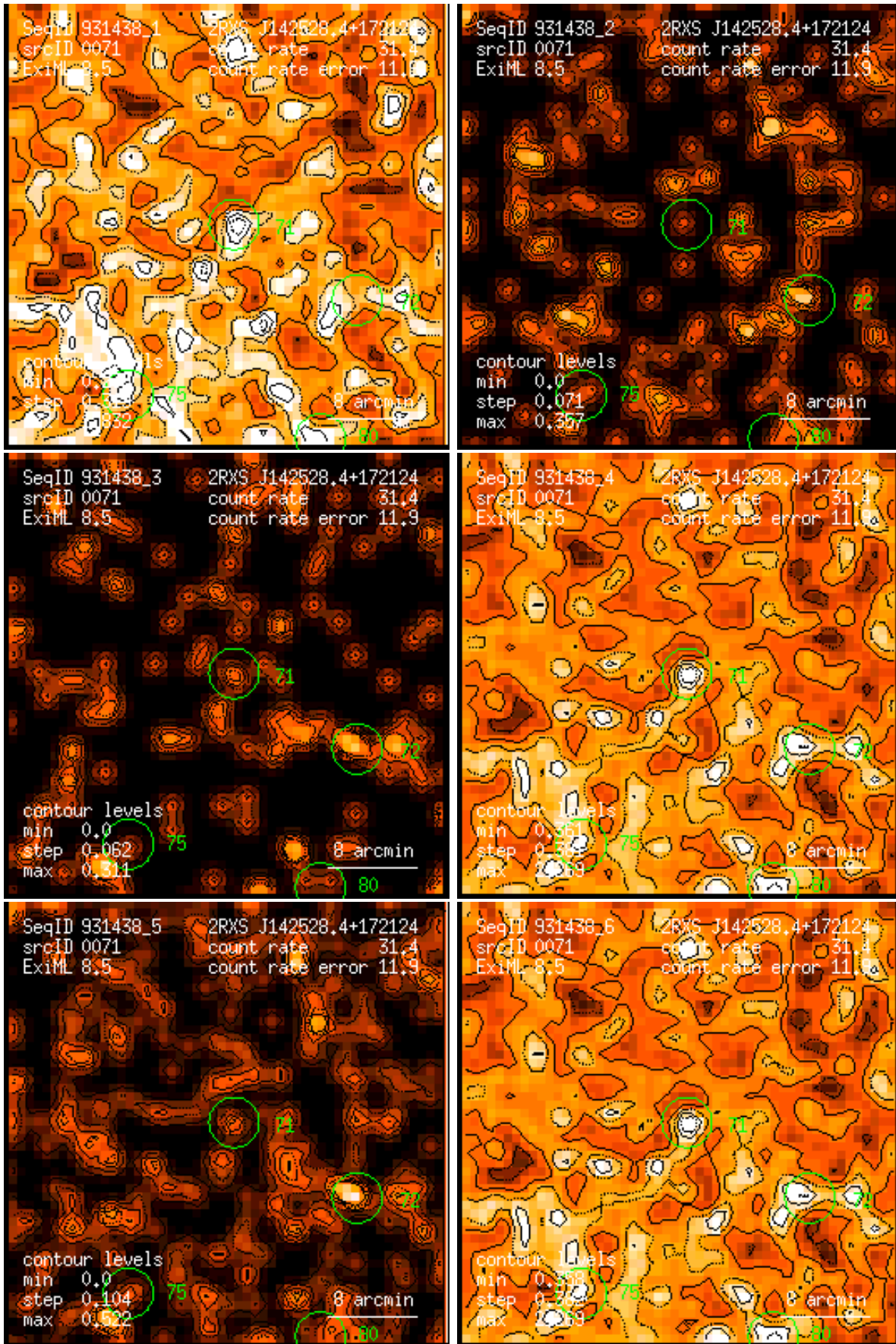
Figure 71: RASS 931438: detection 0071: band rate images, Gaussian filter: (1) PSPC channels 11 – 41, (2) 52 – 90, (3) 91 – 201, (4) 11 – 235, (5) 52 – 201, (6) 11 – 201. Broad band rates in counts/ks. Band rate contour levels in counts/ks/arcmin 2 .
