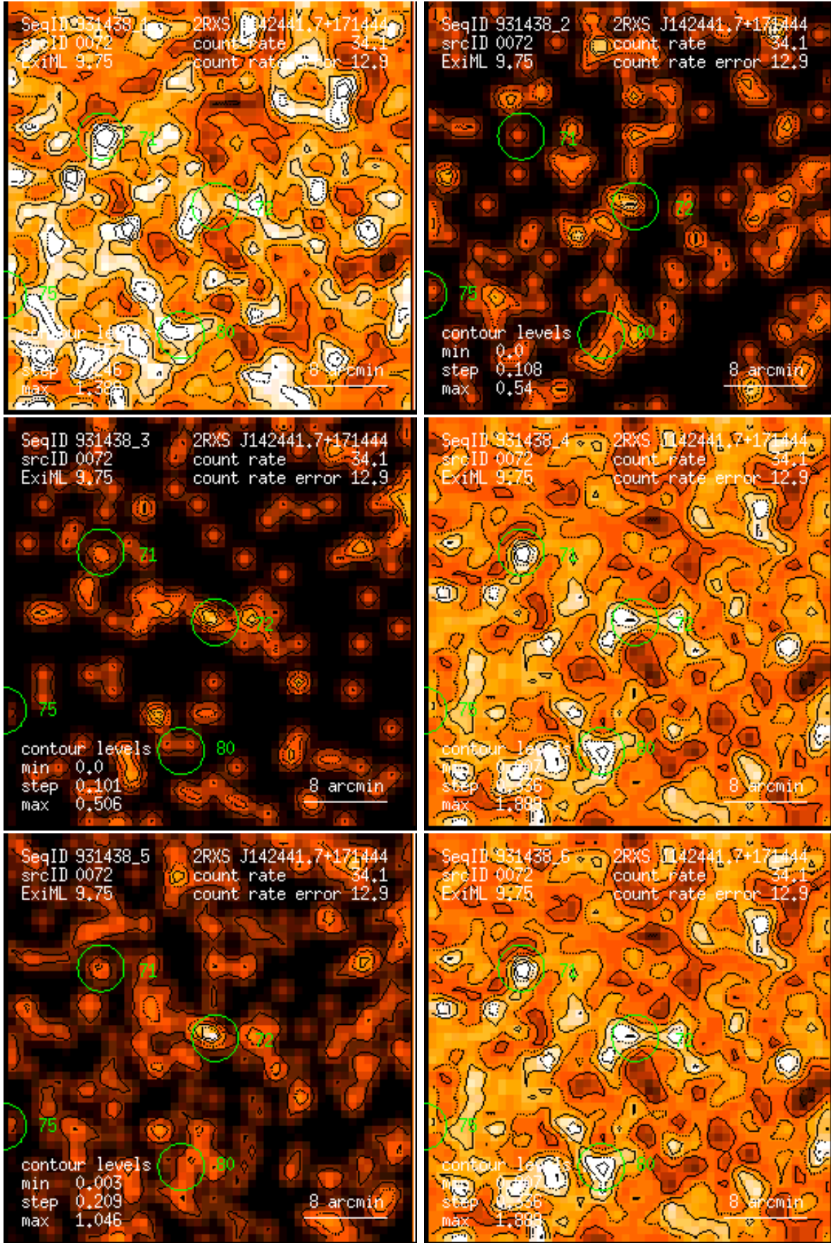
Figure 72: RASS 931438: detection 0072: band rate images, Gaussian filter: (1) PSPC channels 11 – 41, (2) 52 – 90, (3) 91 – 201, (4) 11 – 235, (5) 52 – 201, (6) 11 – 201. Broad band rates in counts/ks. Band rate contour levels in counts/ks/arcmin 2 .
