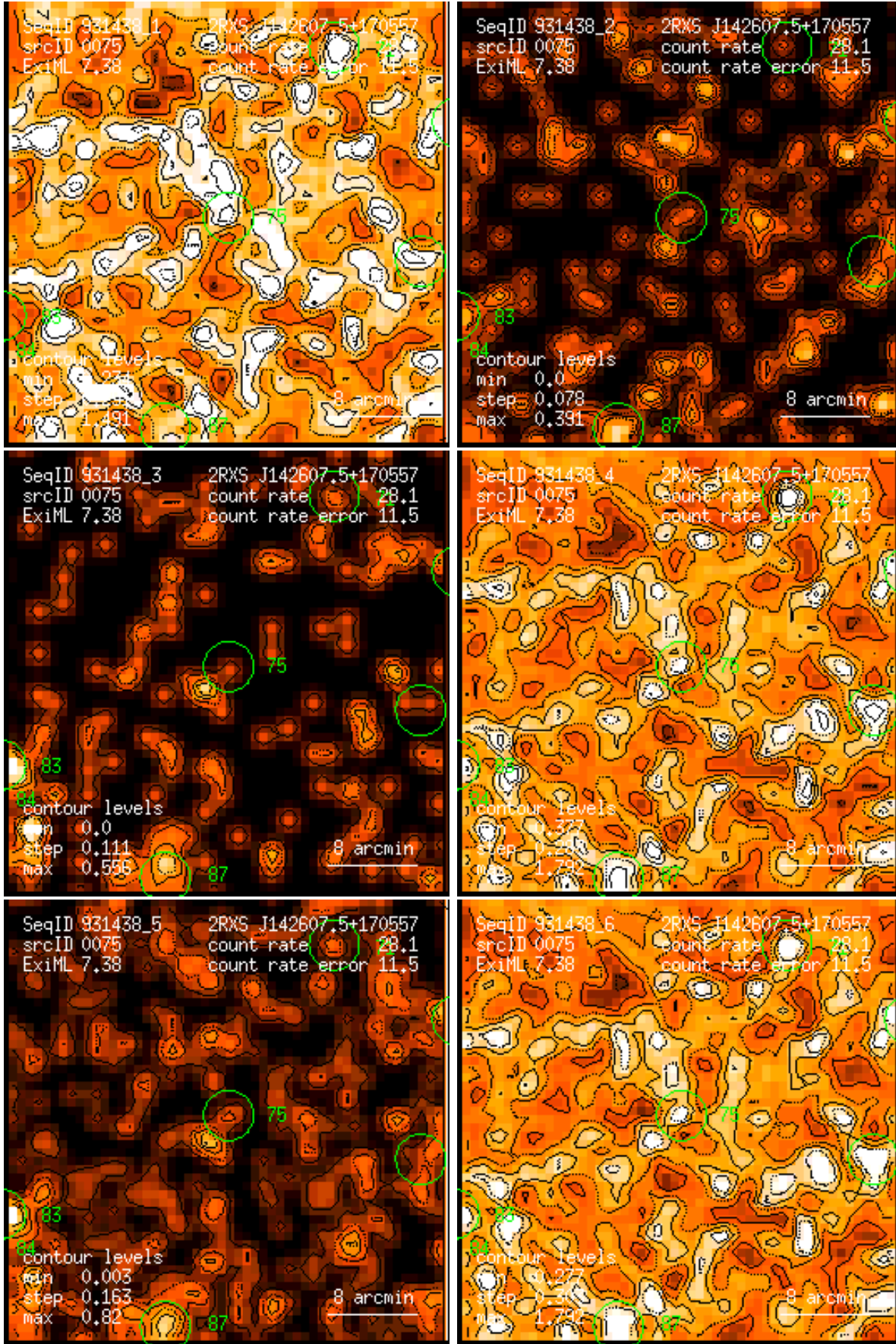
Figure 75: RASS 931438: detection 0075: band rate images, Gaussian filter: (1) PSPC channels 11 – 41, (2) 52 – 90, (3) 91 – 201, (4) 11 – 235, (5) 52 – 201, (6) 11 – 201. Broad band rates in counts/ks. Band rate contour levels in counts/ks/arcmin 2 .
