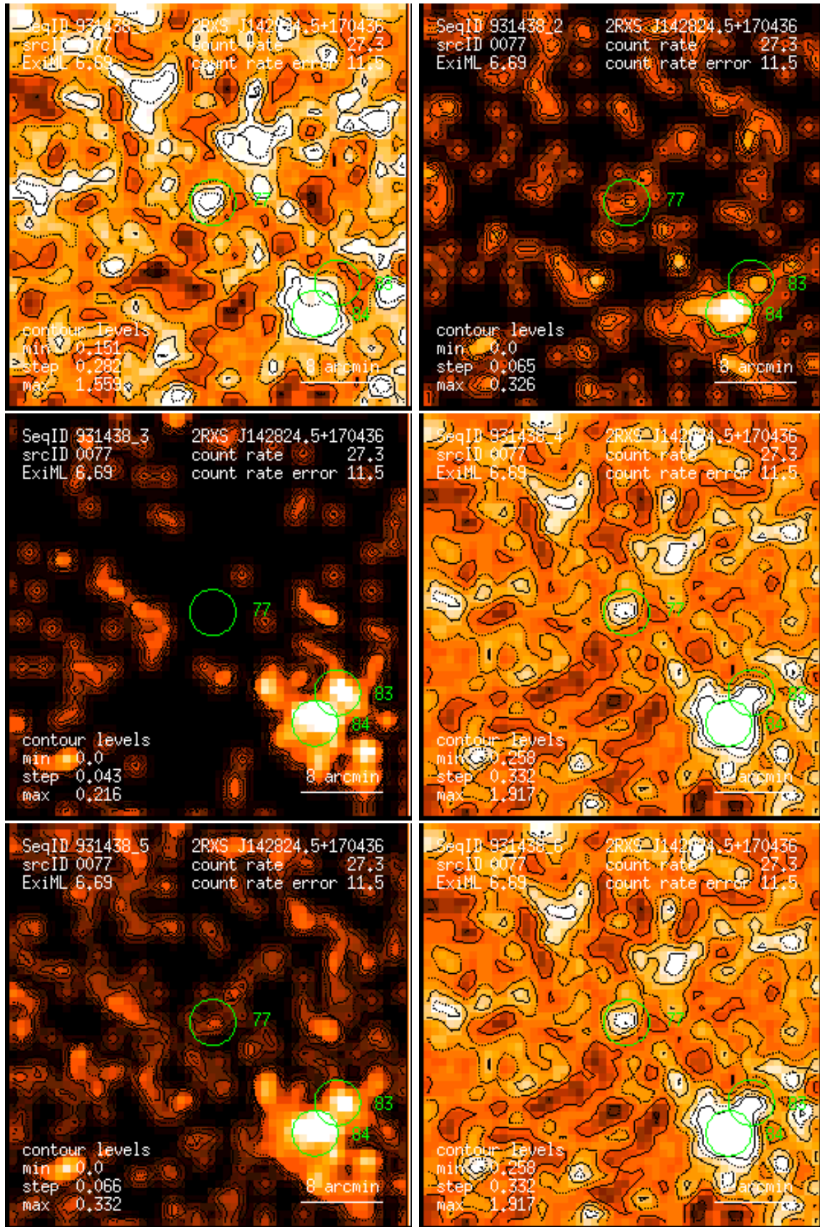
Figure 77: RASS 931438: detection 0077: band rate images, Gaussian filter: (1) PSPC channels 11 – 41, (2) 52 – 90, (3) 91 – 201, (4) 11 – 235, (5) 52 – 201, (6) 11 – 201. Broad band rates in counts/ks. Band rate contour levels in counts/ks/arcmin 2 .
