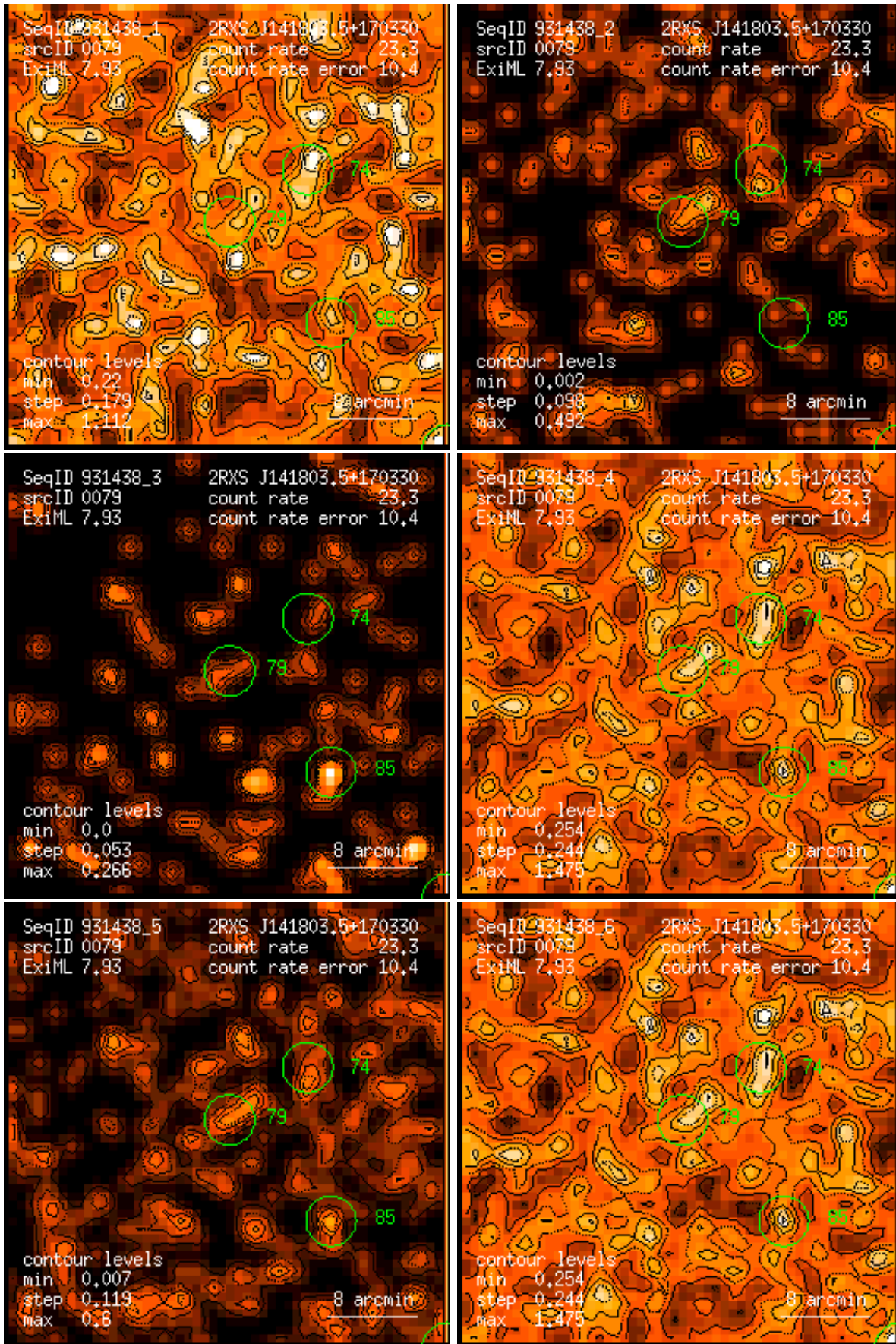
Figure 79: RASS 931438: detection 0079: band rate images, Gaussian filter: (1) PSPC channels 11 – 41, (2) 52 – 90, (3) 91 – 201, (4) 11 – 235, (5) 52 – 201, (6) 11 – 201. Broad band rates in counts/ks. Band rate contour levels in counts/ks/arcmin 2 .
