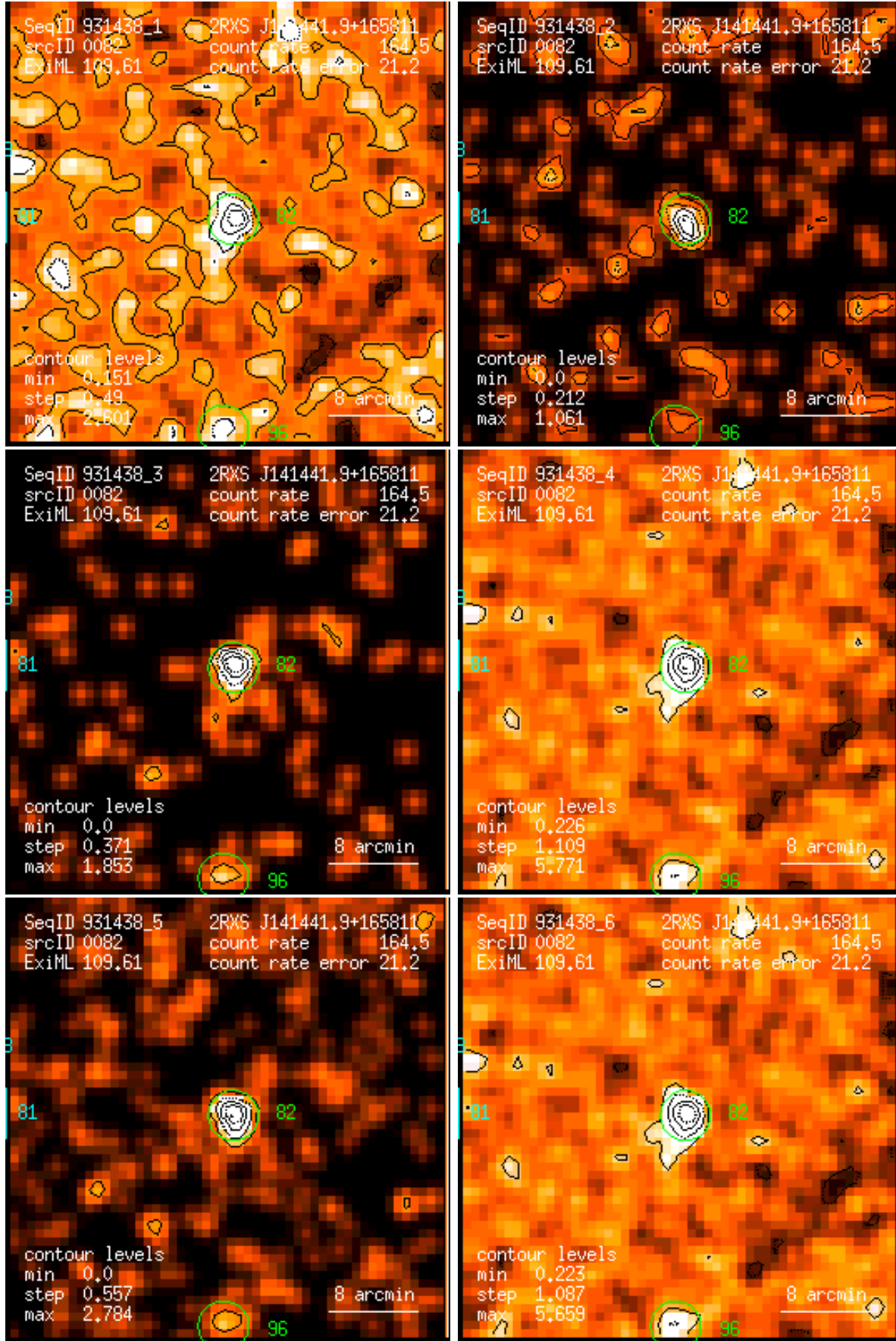
Figure 82: RASS 931438: detection 0082: band rate images, Gaussian filter: (1) PSPC channels 11 – 41, (2) 52 – 90, (3) 91 – 201, (4) 11 – 235, (5) 52 – 201, (6) 11 – 201. Broad band rates in counts/ks. Band rate contour levels in counts/ks/arcmin 2 .
