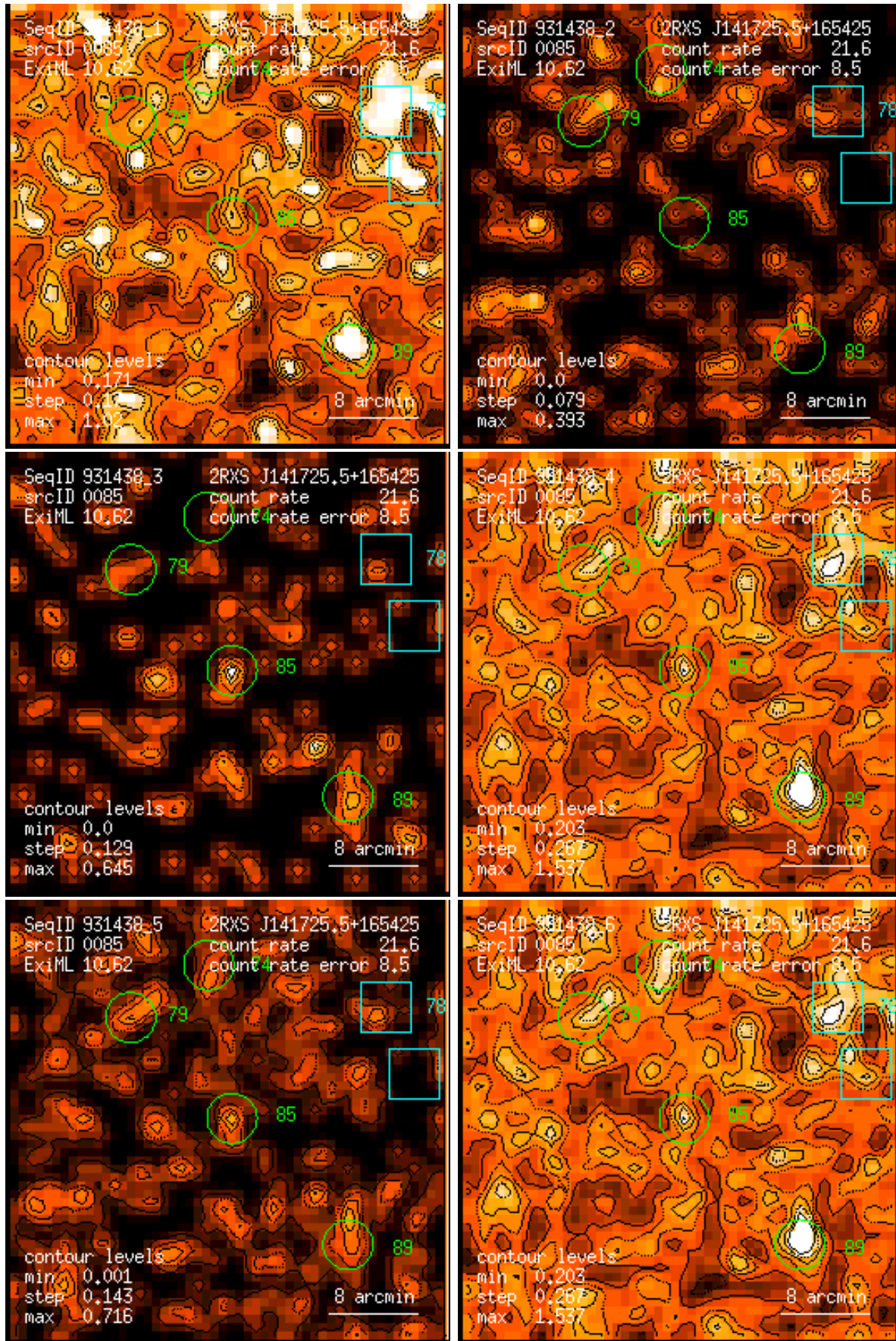
Figure 85: RASS 931438: detection 0085: band rate images, Gaussian filter: (1) PSPC channels 11 – 41, (2) 52 – 90, (3) 91 – 201, (4) 11 – 235, (5) 52 – 201, (6) 11 – 201. Broad band rates in counts/ks. Band rate contour levels in counts/ks/arcmin 2 .
