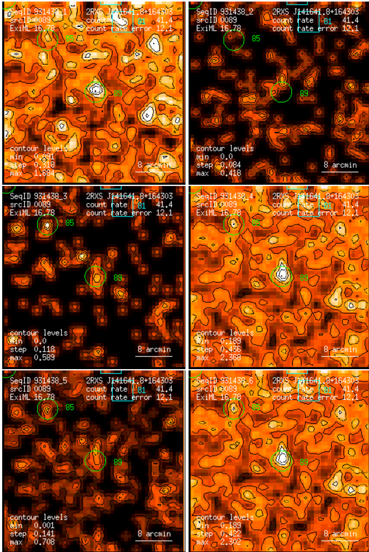
Figure 89: RASS 931438: detection 0089: band rate images, Gaussian filter: (1) PSPC channels 11 – 41, (2) 52 – 90, (3) 91 – 201, (4) 11 – 235, (5) 52 – 201, (6) 11 – 201. Broad band rates in counts/ks. Band rate contour levels in counts/ks/arcmin 2 .
