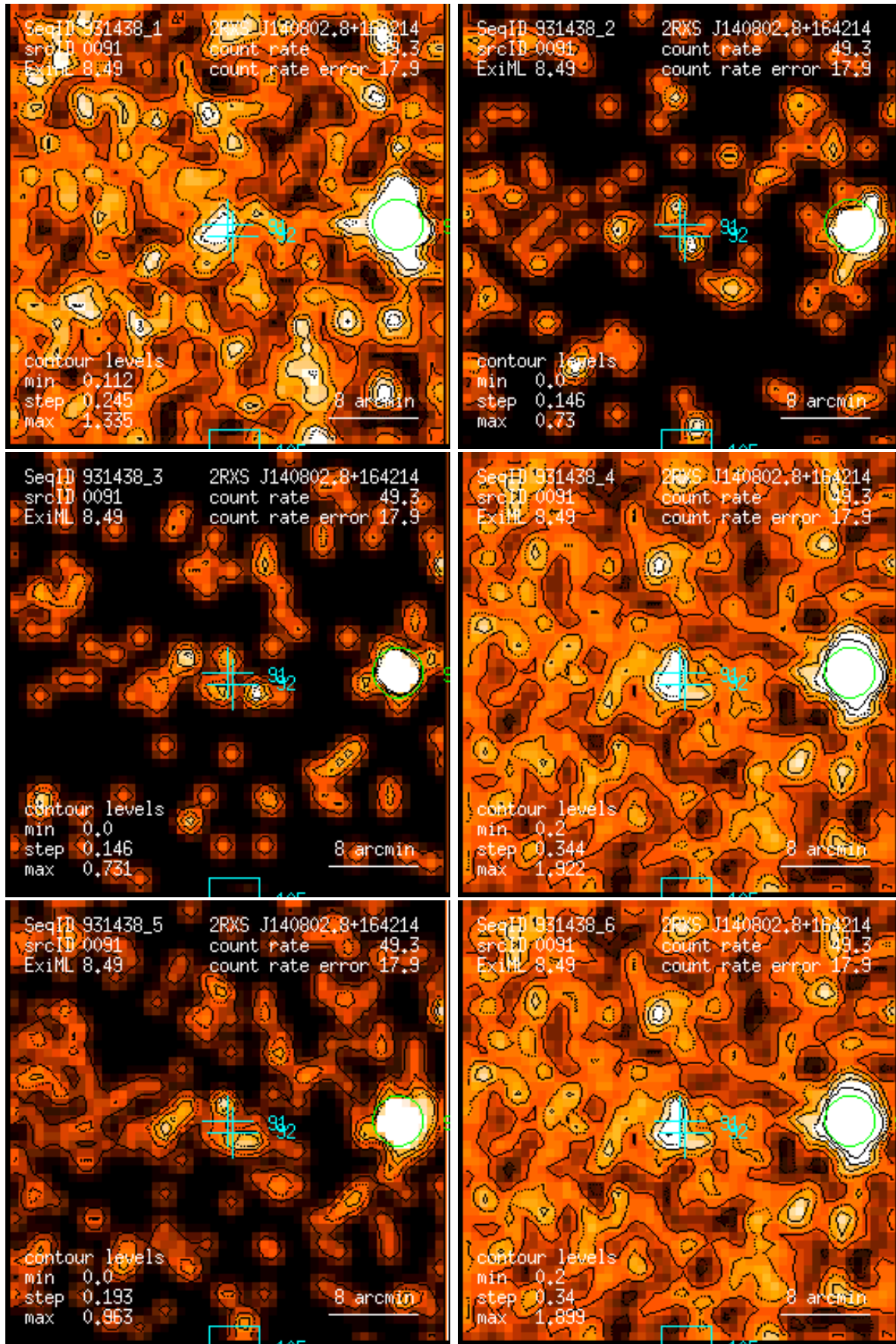
Figure 91: RASS 931438: detection 0091: band rate images, Gaussian filter: (1) PSPC channels 11 – 41, (2) 52 – 90, (3) 91 – 201, (4) 11 – 235, (5) 52 – 201, (6) 11 – 201. Broad band rates in counts/ks. Band rate contour levels in counts/ks/arcmin 2 .
