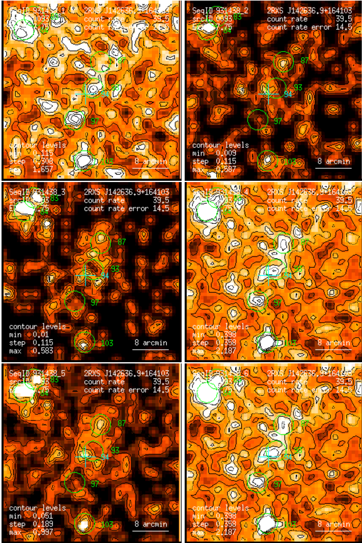
Figure 93: RASS 931438: detection 0093: band rate images, Gaussian filter: (1) PSPC channels 11 – 41, (2) 52 – 90, (3) 91 – 201, (4) 11 – 235, (5) 52 – 201, (6) 11 – 201. Broad band rates in counts/ks. Band rate contour levels in counts/ks/arcmin 2 .
