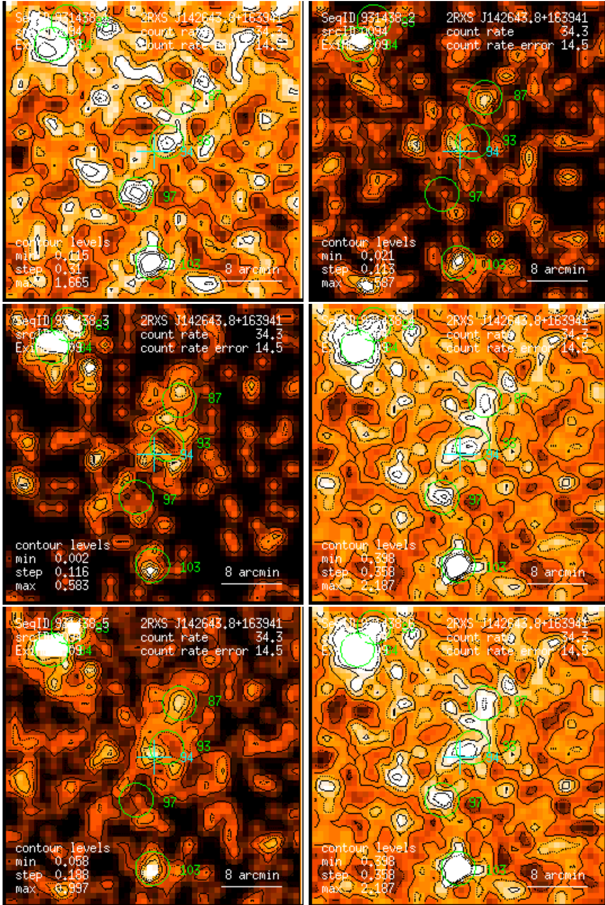
Figure 94: RASS 931438: detection 0094: band rate images, Gaussian filter: (1) PSPC channels 11 – 41, (2) 52 – 90, (3) 91 – 201, (4) 11 – 235, (5) 52 – 201, (6) 11 – 201. Broad band rates in counts/ks. Band rate contour levels in counts/ks/arcmin 2 .
