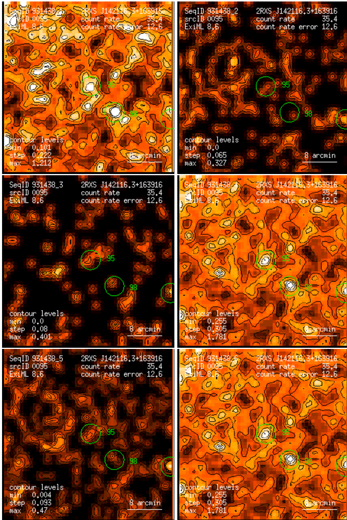
Figure 95: RASS 931438: detection 0095: band rate images, Gaussian filter: (1) PSPC channels 11 – 41, (2) 52 – 90, (3) 91 – 201, (4) 11 – 235, (5) 52 – 201, (6) 11 – 201. Broad band rates in counts/ks. Band rate contour levels in counts/ks/arcmin 2 .
