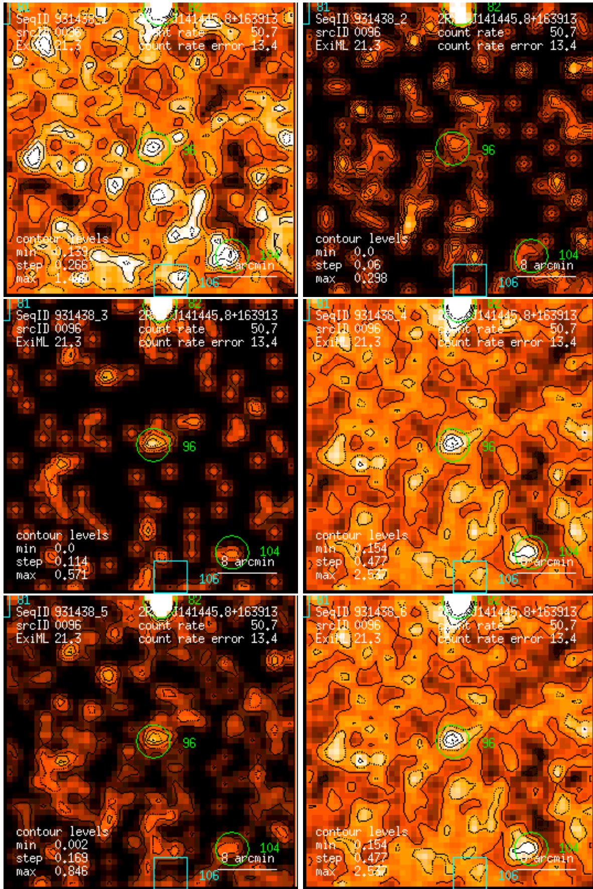
Figure 96: RASS 931438: detection 0096: band rate images, Gaussian filter: (1) PSPC channels 11 – 41, (2) 52 – 90, (3) 91 – 201, (4) 11 – 235, (5) 52 – 201, (6) 11 – 201. Broad band rates in counts/ks. Band rate contour levels in counts/ks/arcmin 2 .
