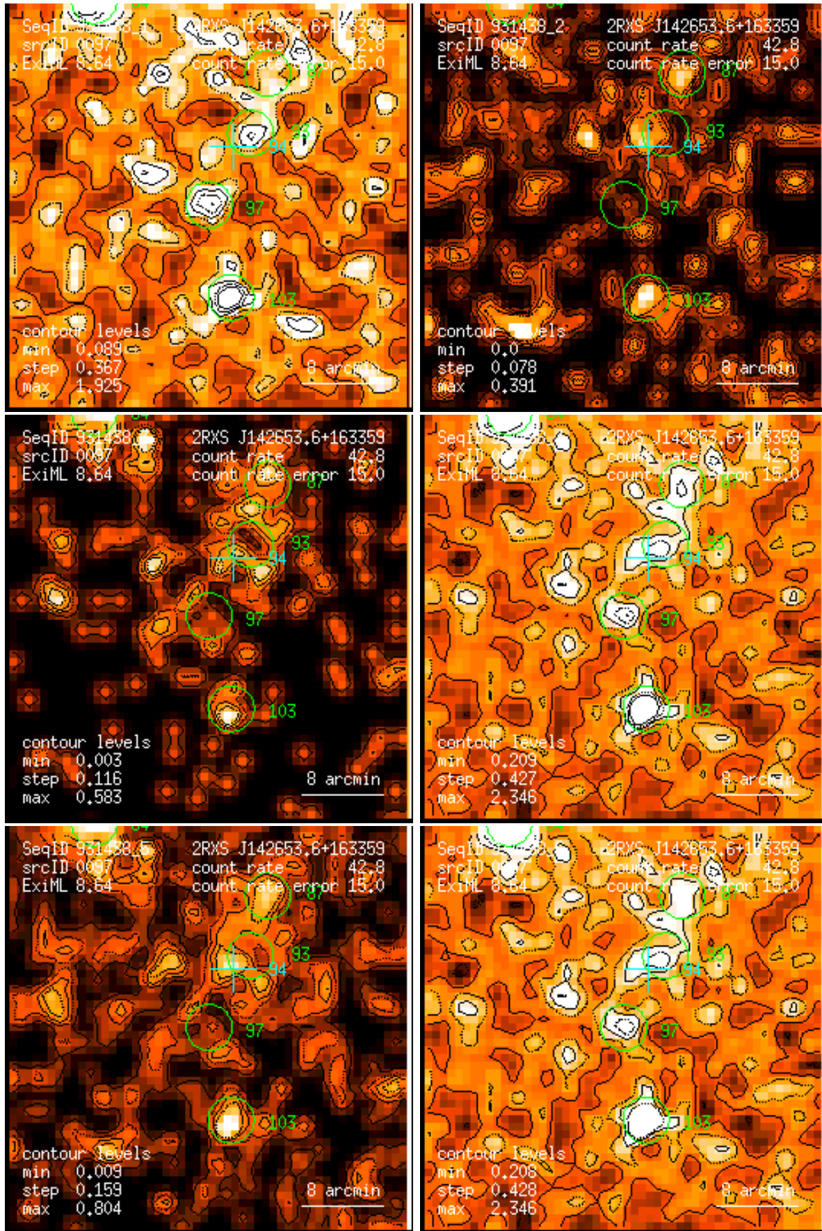
Figure 97: RASS 931438: detection 0097: band rate images, Gaussian filter: (1) PSPC channels 11 – 41, (2) 52 – 90, (3) 91 – 201, (4) 11 – 235, (5) 52 – 201, (6) 11 – 201. Broad band rates in counts/ks. Band rate contour levels in counts/ks/arcmin 2 .
