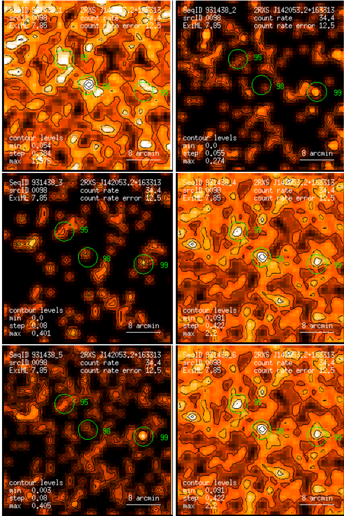
Figure 98: RASS 931438: detection 0098: band rate images, Gaussian filter: (1) PSPC channels 11 – 41, (2) 52 – 90, (3) 91 – 201, (4) 11 – 235, (5) 52 – 201, (6) 11 – 201. Broad band rates in counts/ks. Band rate contour levels in counts/ks/arcmin 2 .
