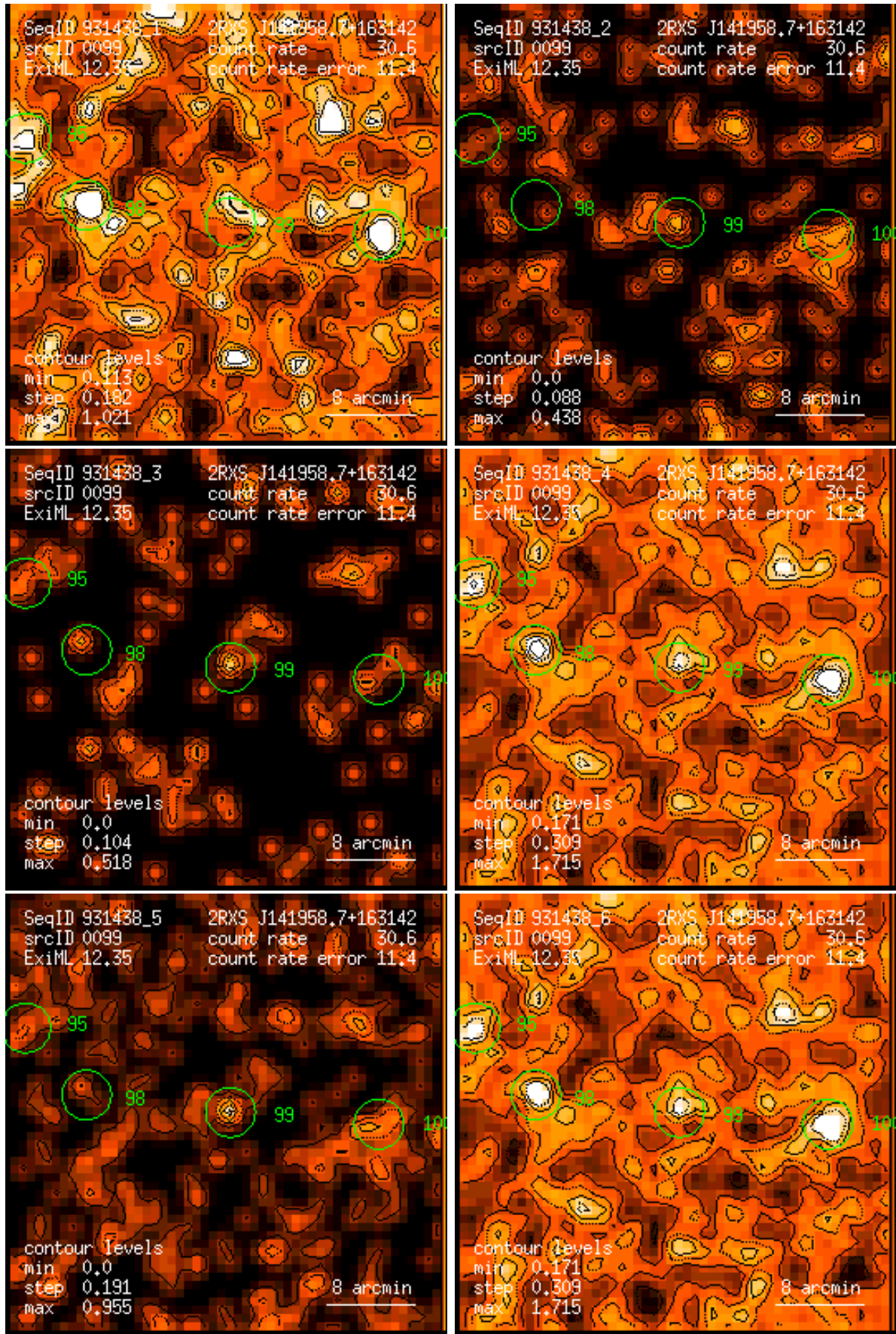
Figure 99: RASS 931438: detection 0099: band rate images, Gaussian filter: (1) PSPC channels 11 – 41, (2) 52 – 90, (3) 91 – 201, (4) 11 – 235, (5) 52 – 201, (6) 11 – 201. Broad band rates in counts/ks. Band rate contour levels in counts/ks/arcmin 2 .
