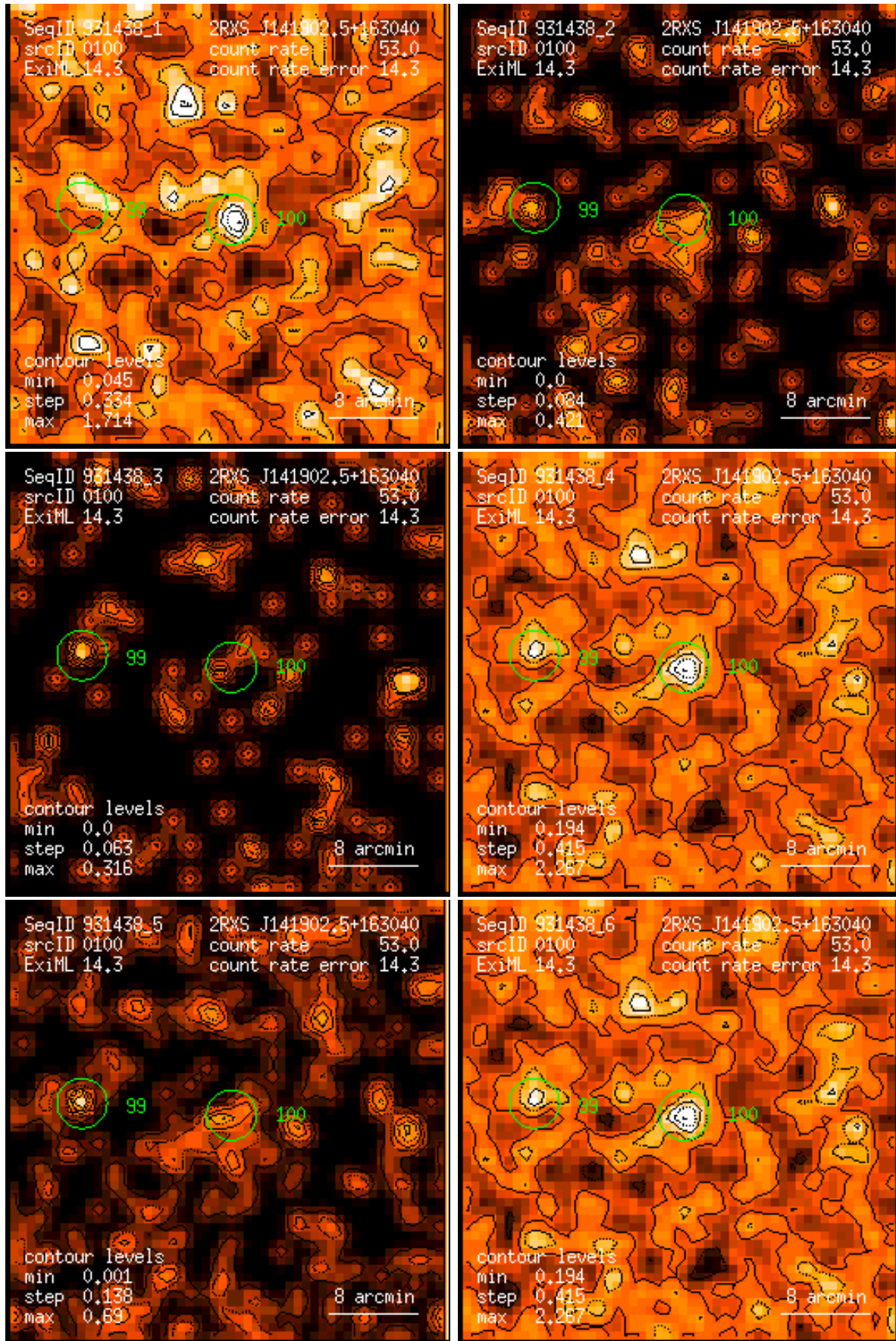
Figure 100: RASS 931438: detection 0100: band rate images, Gaussian filter: (1) PSPC channels 11 – 41, (2) 52 – 90, (3) 91 – 201, (4) 11 – 235, (5) 52 – 201, (6) 11 – 201. Broad band rates in counts/ks. Band rate contour levels in counts/ks/arcmin 2 .
