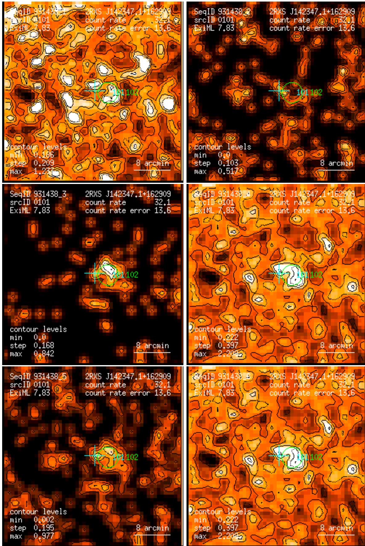
Figure 101: RASS 931438: detection 0101: band rate images, Gaussian filter: (1) PSPC channels 11 – 41, (2) 52 – 90, (3) 91 – 201, (4) 11 – 235, (5) 52 – 201, (6) 11 – 201. Broad band rates in counts/ks. Band rate contour levels in counts/ks/arcmin 2 .
