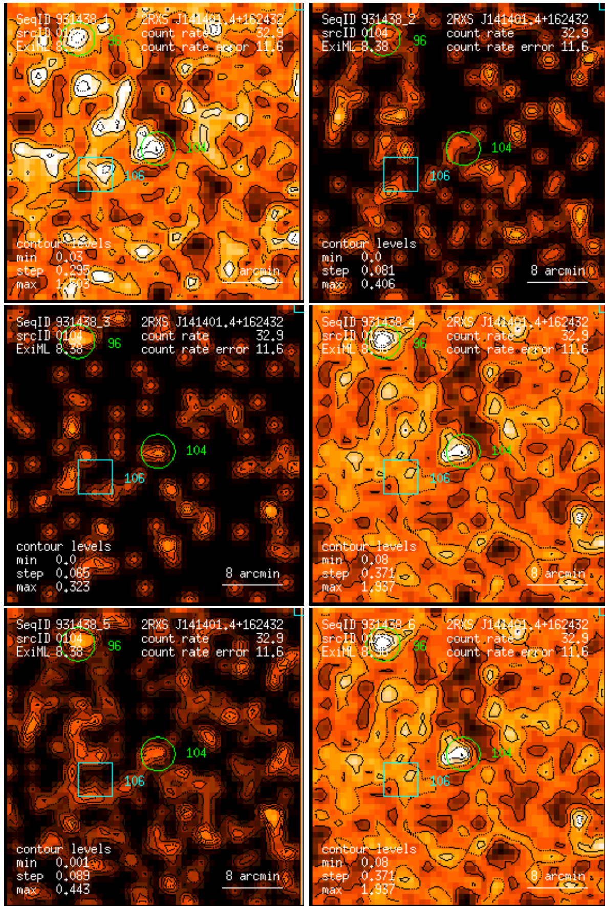
Figure 104: RASS 931438: detection 0104: band rate images, Gaussian filter: (1) PSPC channels 11 – 41, (2) 52 – 90, (3) 91 – 201, (4) 11 – 235, (5) 52 – 201, (6) 11 – 201. Broad band rates in counts/ks. Band rate contour levels in counts/ks/arcmin 2 .
