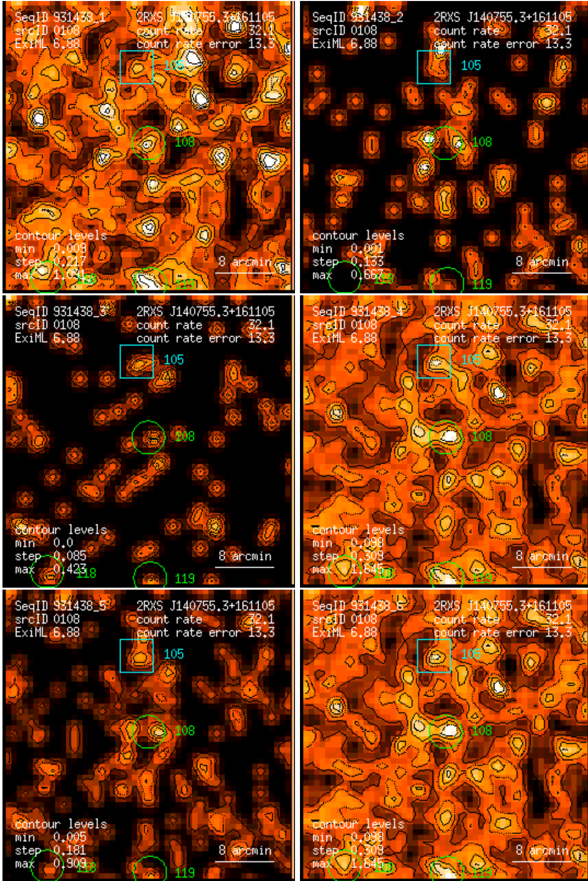
Figure 108: RASS 931438: detection 0108: band rate images, Gaussian filter: (1) PSPC channels 11 – 41, (2) 52 – 90, (3) 91 – 201, (4) 11 – 235, (5) 52 – 201, (6) 11 – 201. Broad band rates in counts/ks. Band rate contour levels in counts/ks/arcmin 2 .
