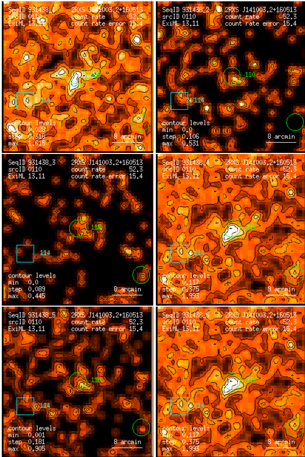
Figure 110: RASS 931438: detection 0110: band rate images, Gaussian filter: (1) PSPC channels 11 – 41, (2) 52 – 90, (3) 91 – 201, (4) 11 – 235, (5) 52 – 201, (6) 11 – 201. Broad band rates in counts/ks. Band rate contour levels in counts/ks/arcmin 2 .
