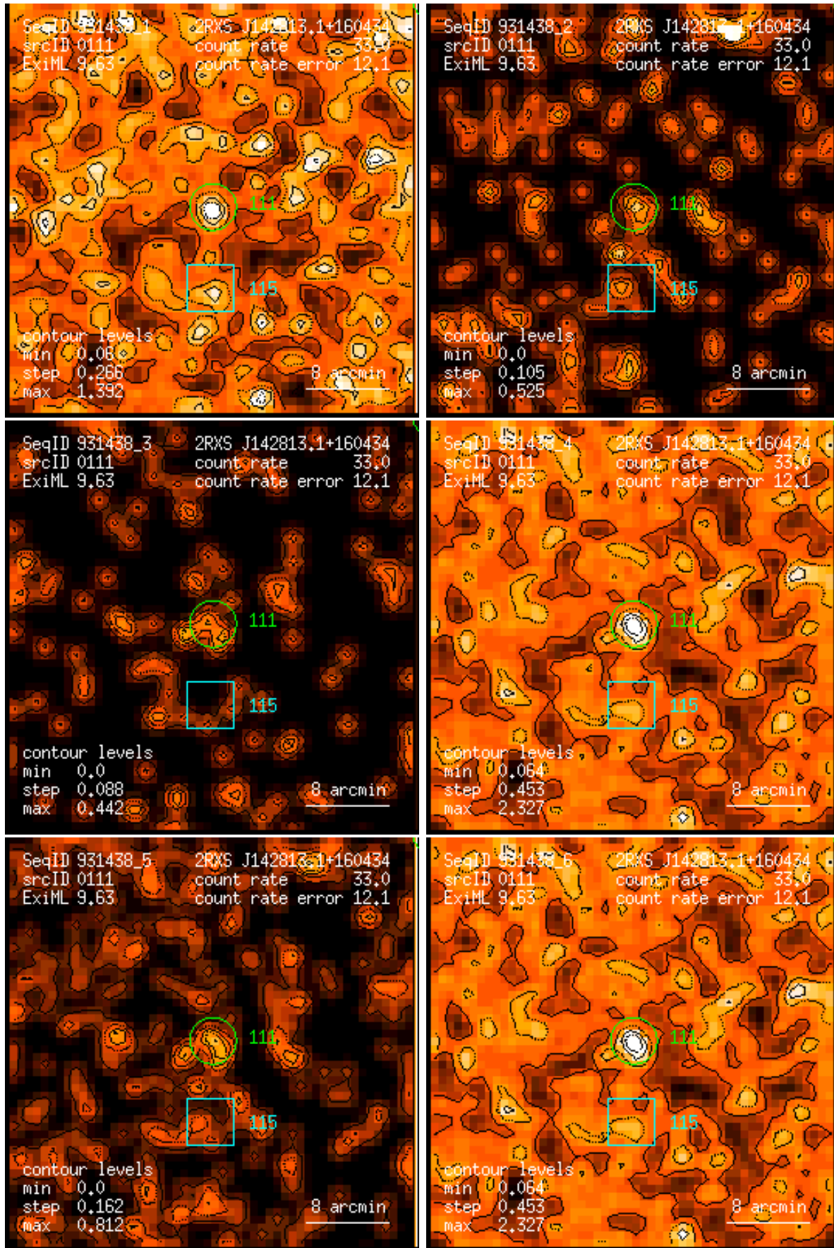
Figure 111: RASS 931438: detection 0111: band rate images, Gaussian filter: (1) PSPC channels 11 – 41, (2) 52 – 90, (3) 91 – 201, (4) 11 – 235, (5) 52 – 201, (6) 11 – 201. Broad band rates in counts/ks. Band rate contour levels in counts/ks/arcmin 2 .
