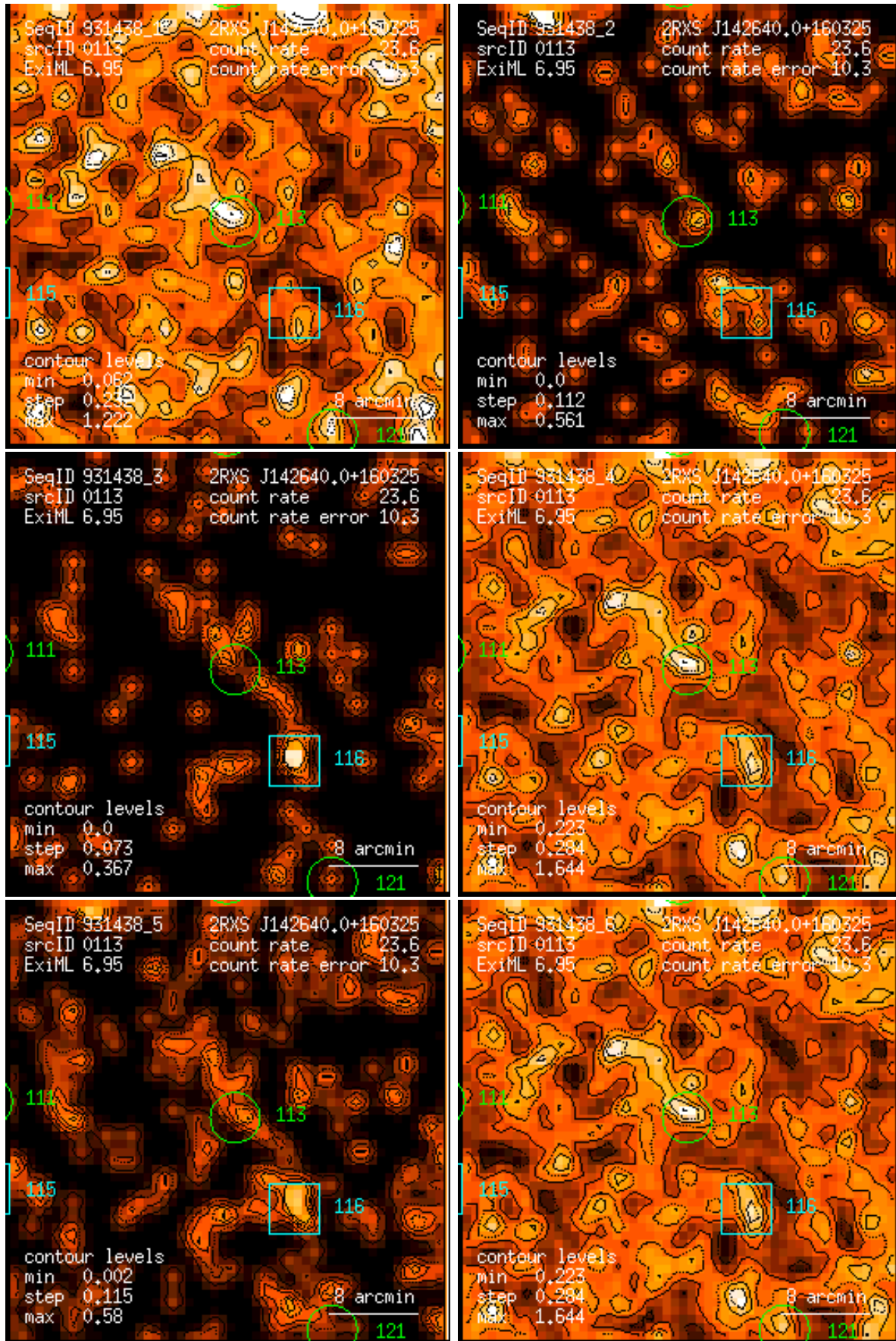
Figure 113: RASS 931438: detection 0113: band rate images, Gaussian filter: (1) PSPC channels 11 – 41, (2) 52 – 90, (3) 91 – 201, (4) 11 – 235, (5) 52 – 201, (6) 11 – 201. Broad band rates in counts/ks. Band rate contour levels in counts/ks/arcmin 2 .
