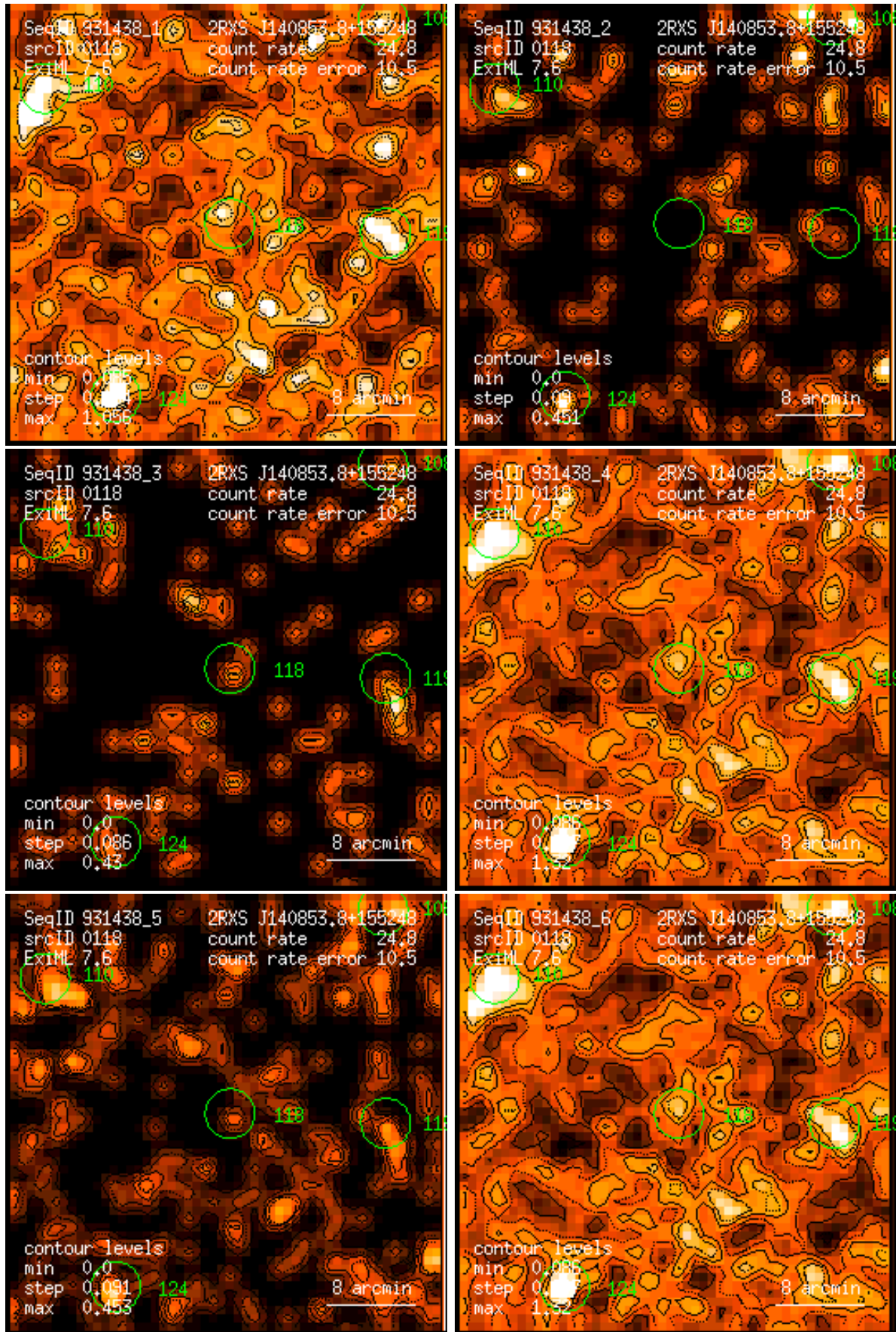
Figure 118: RASS 931438: detection 0118: band rate images, Gaussian filter: (1) PSPC channels 11 – 41, (2) 52 – 90, (3) 91 – 201, (4) 11 – 235, (5) 52 – 201, (6) 11 – 201. Broad band rates in counts/ks. Band rate contour levels in counts/ks/arcmin 2 .
