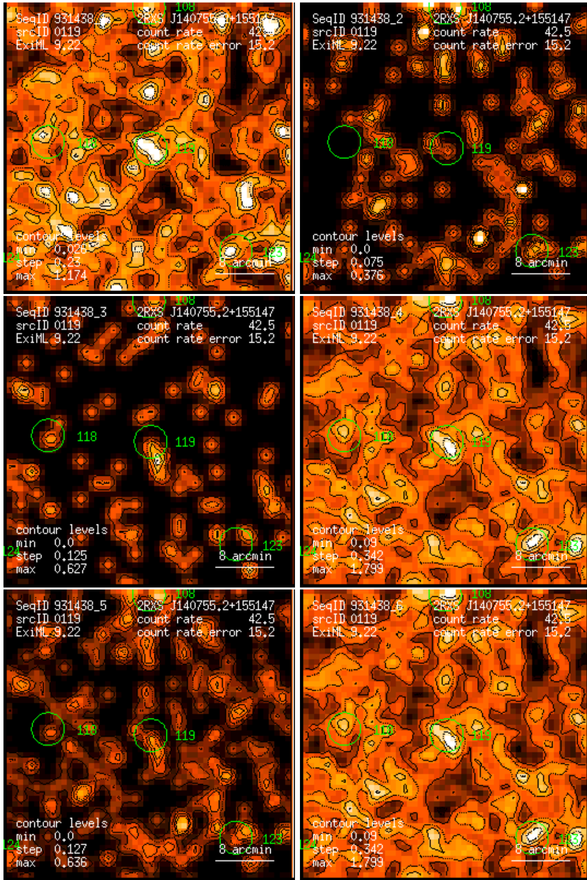
Figure 119: RASS 931438: detection 0119: band rate images, Gaussian filter: (1) PSPC channels 11 – 41, (2) 52 – 90, (3) 91 – 201, (4) 11 – 235, (5) 52 – 201, (6) 11 – 201. Broad band rates in counts/ks. Band rate contour levels in counts/ks/arcmin 2 .
