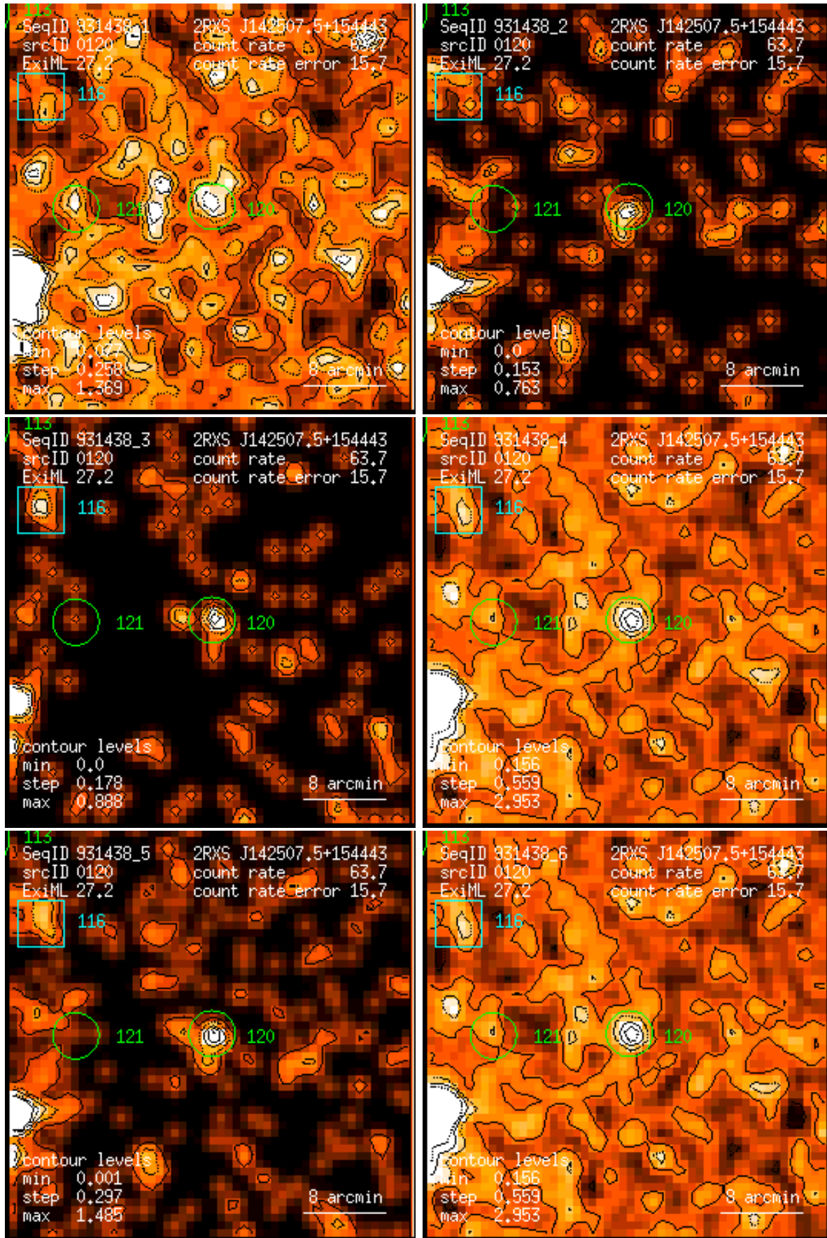
Figure 120: RASS 931438: detection 0120: band rate images, Gaussian filter: (1) PSPC channels 11 – 41, (2) 52 – 90, (3) 91 – 201, (4) 11 – 235, (5) 52 – 201, (6) 11 – 201. Broad band rates in counts/ks. Band rate contour levels in counts/ks/arcmin 2 .
