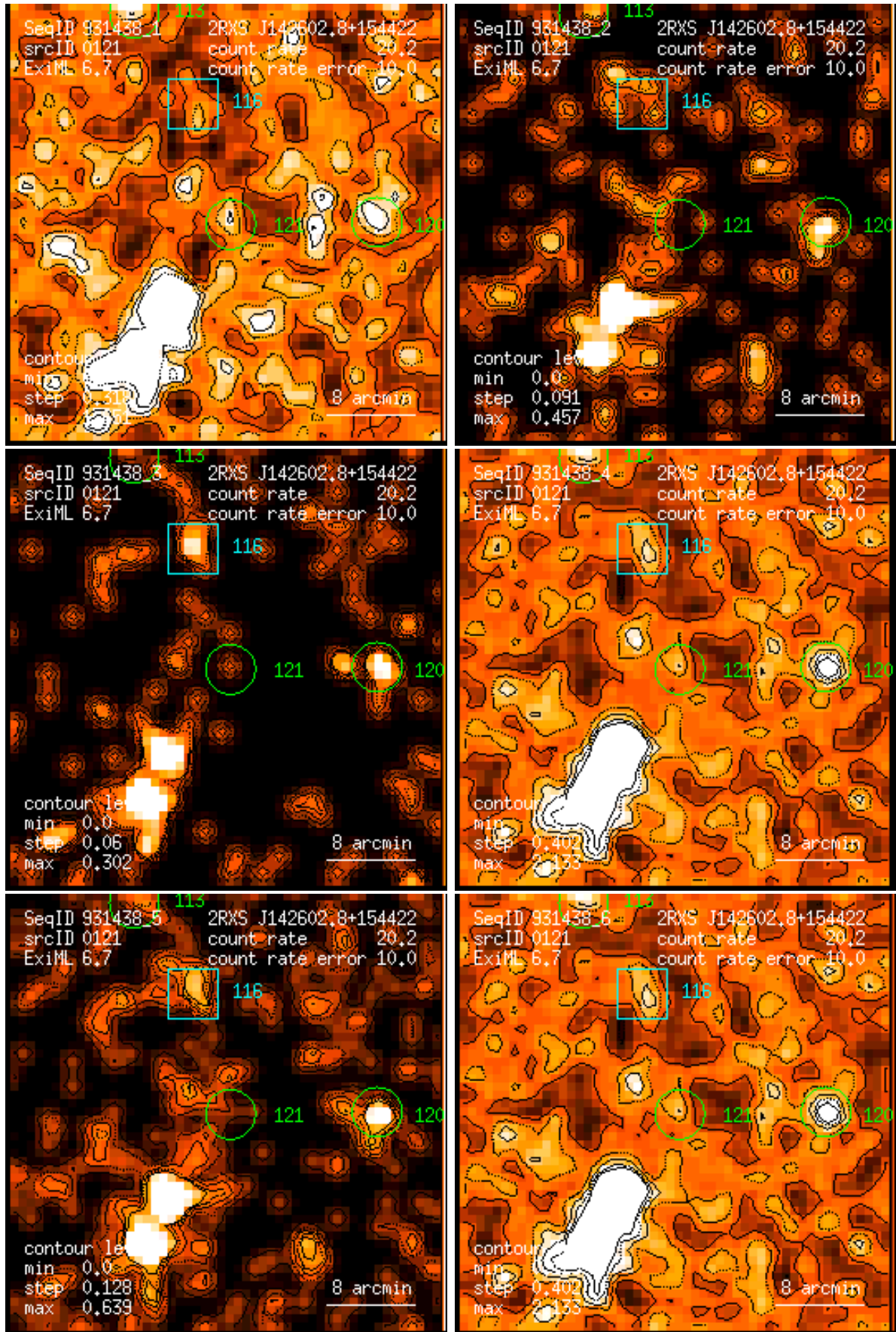
Figure 121: RASS 931438: detection 0121: band rate images, Gaussian filter: (1) PSPC channels 11 – 41, (2) 52 – 90, (3) 91 – 201, (4) 11 – 235, (5) 52 – 201, (6) 11 – 201. Broad band rates in counts/ks. Band rate contour levels in counts/ks/arcmin 2 .
