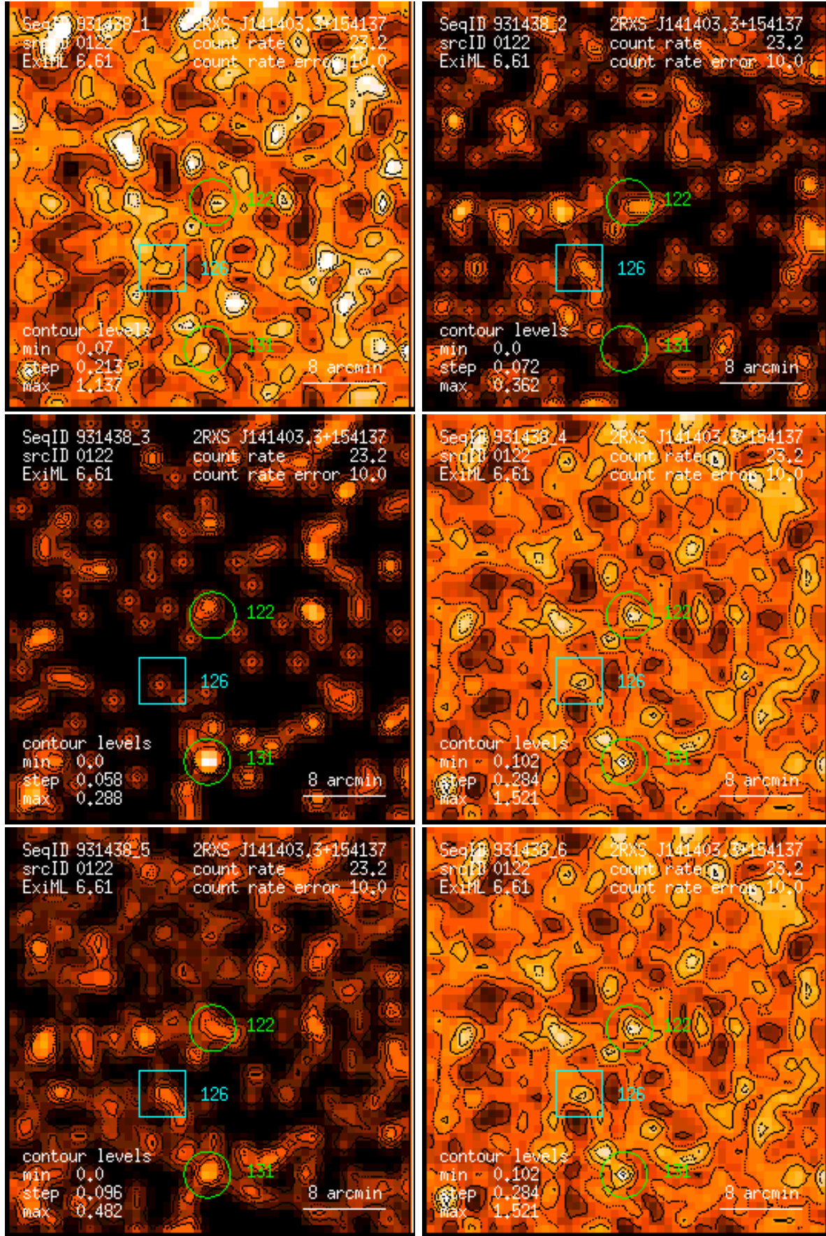
Figure 122: RASS 931438: detection 0122: band rate images, Gaussian filter: (1) PSPC channels 11 – 41, (2) 52 – 90, (3) 91 – 201, (4) 11 – 235, (5) 52 – 201, (6) 11 – 201. Broad band rates in counts/ks. Band rate contour levels in counts/ks/arcmin 2 .
