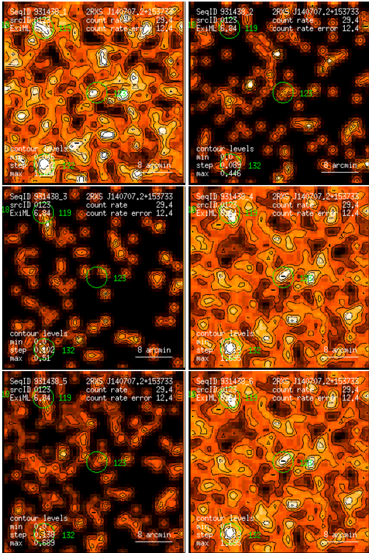
Figure 123: RASS 931438: detection 0123: band rate images, Gaussian filter: (1) PSPC channels 11 – 41, (2) 52 – 90, (3) 91 – 201, (4) 11 – 235, (5) 52 – 201, (6) 11 – 201. Broad band rates in counts/ks. Band rate contour levels in counts/ks/arcmin 2 .
