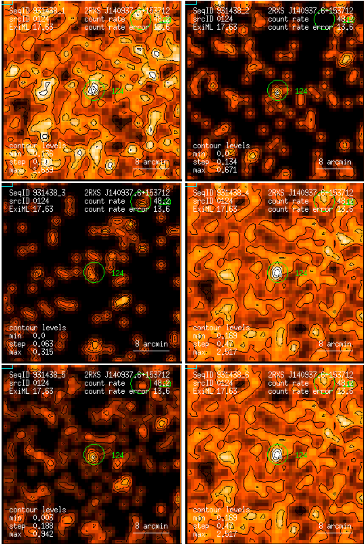
Figure 124: RASS 931438: detection 0124: band rate images, Gaussian filter: (1) PSPC channels 11 – 41, (2) 52 – 90, (3) 91 – 201, (4) 11 – 235, (5) 52 – 201, (6) 11 – 201. Broad band rates in counts/ks. Band rate contour levels in counts/ks/arcmin 2 .
