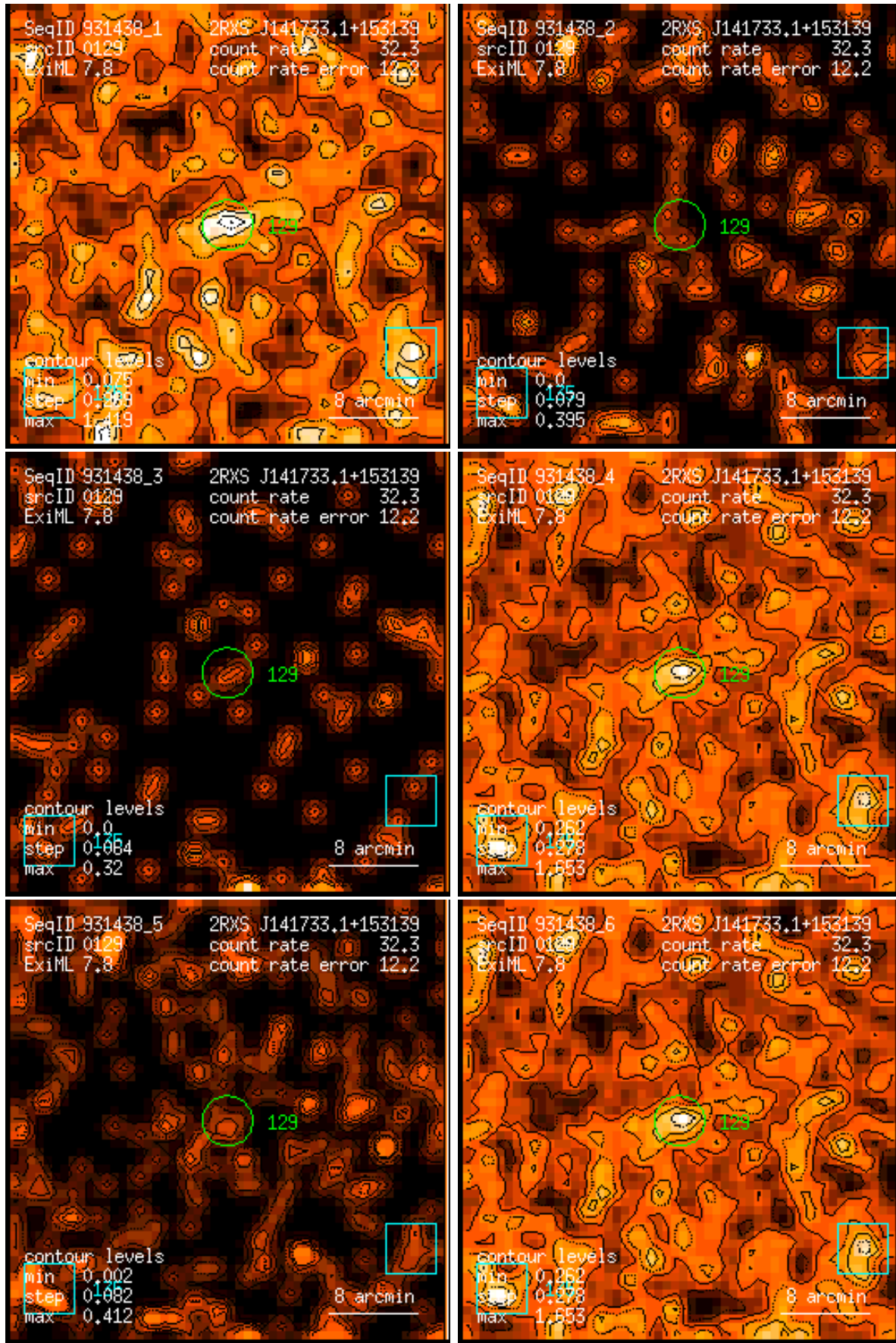
Figure 129: RASS 931438: detection 0129: band rate images, Gaussian filter: (1) PSPC channels 11 – 41, (2) 52 – 90, (3) 91 – 201, (4) 11 – 235, (5) 52 – 201, (6) 11 – 201. Broad band rates in counts/ks. Band rate contour levels in counts/ks/arcmin 2 .
