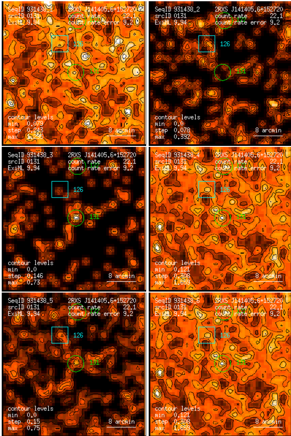
Figure 131: RASS 931438: detection 0131: band rate images, Gaussian filter: (1) PSPC channels 11 – 41, (2) 52 – 90, (3) 91 – 201, (4) 11 – 235, (5) 52 – 201, (6) 11 – 201. Broad band rates in counts/ks. Band rate contour levels in counts/ks/arcmin 2 .
