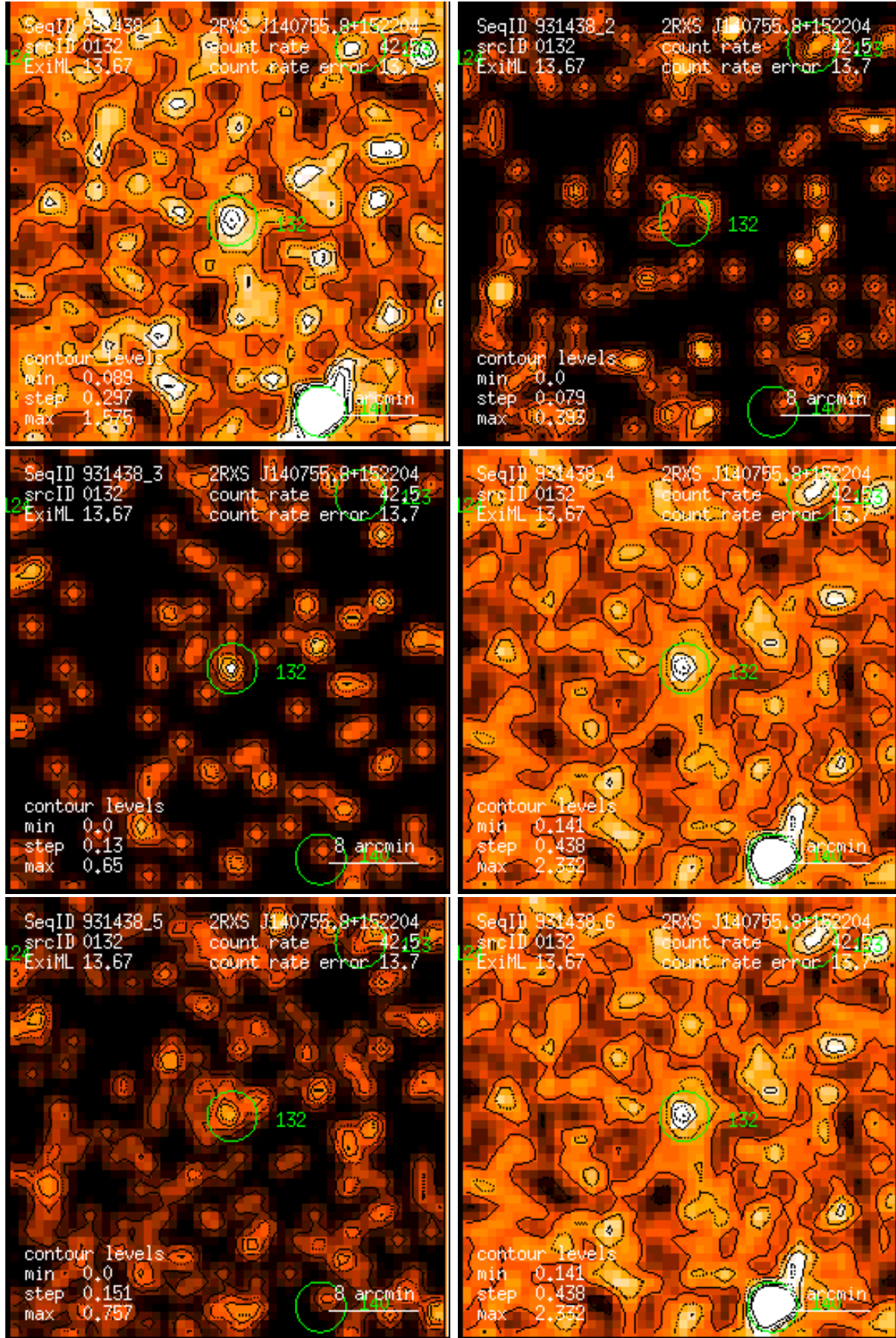
Figure 132: RASS 931438: detection 0132: band rate images, Gaussian filter: (1) PSPC channels 11 – 41, (2) 52 – 90, (3) 91 – 201, (4) 11 – 235, (5) 52 – 201, (6) 11 – 201. Broad band rates in counts/ks. Band rate contour levels in counts/ks/arcmin 2 .
