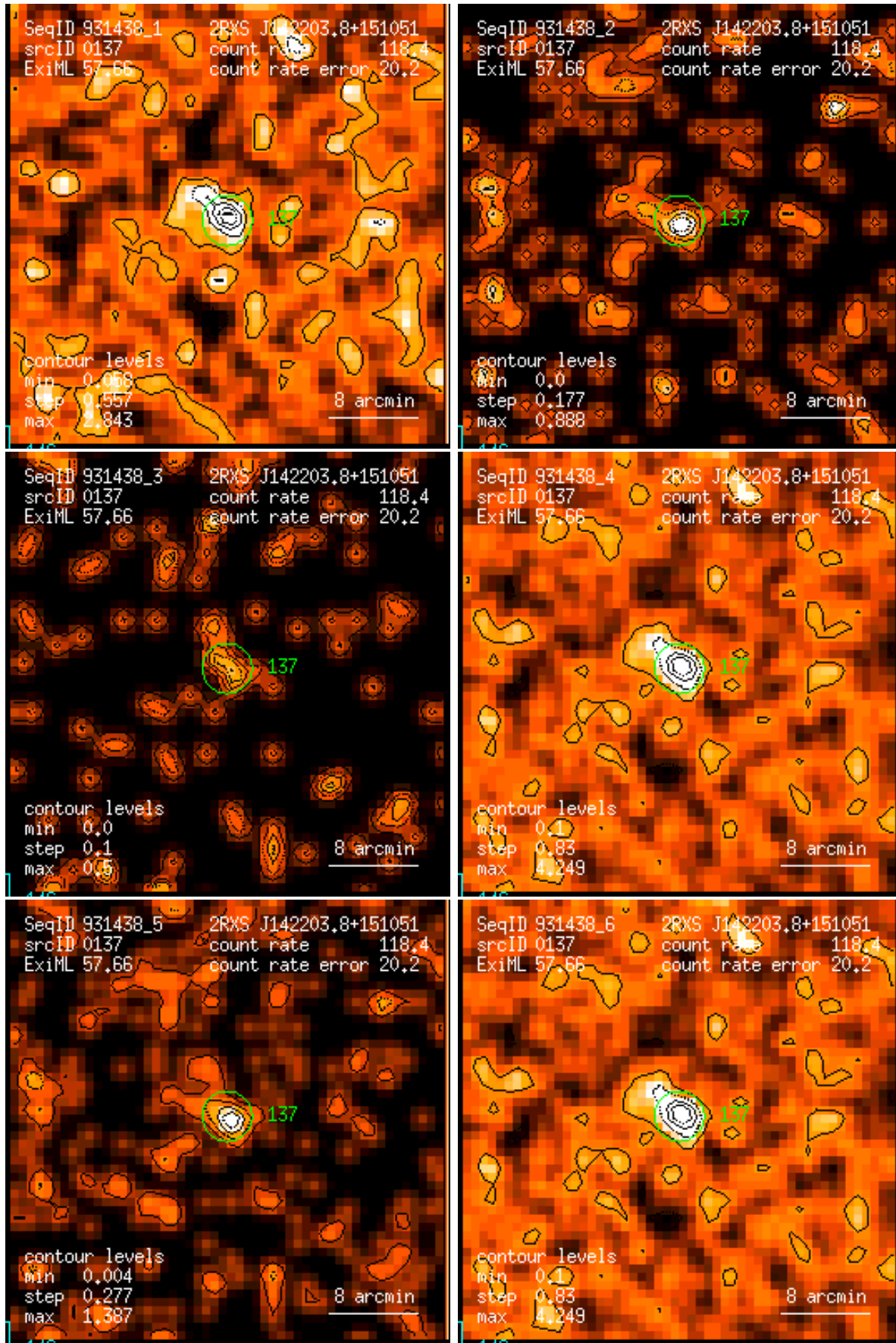
Figure 137: RASS 931438: detection 0137: band rate images, Gaussian filter: (1) PSPC channels 11 – 41, (2) 52 – 90, (3) 91 – 201, (4) 11 – 235, (5) 52 – 201, (6) 11 – 201. Broad band rates in counts/ks. Band rate contour levels in counts/ks/arcmin 2 .
