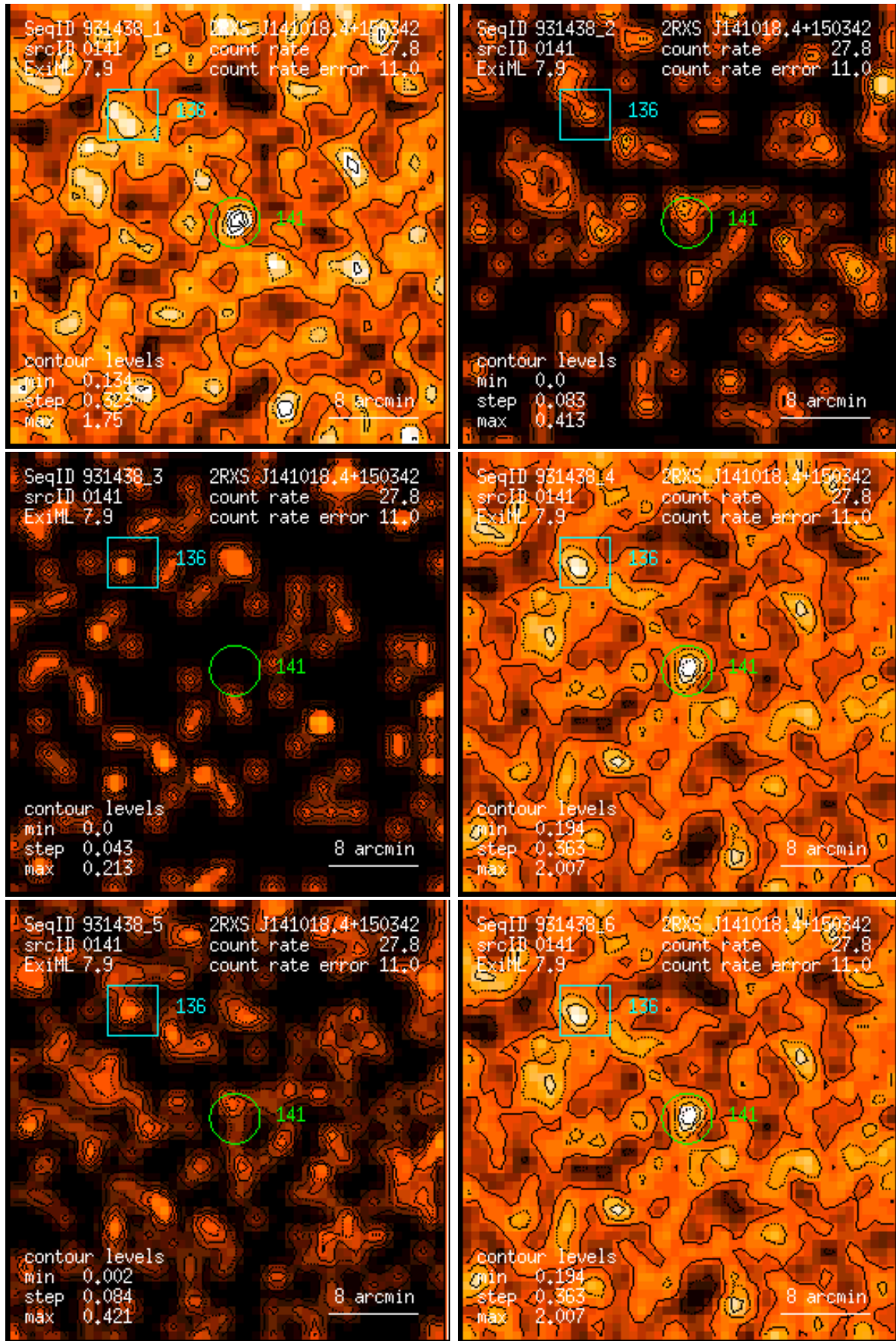
Figure 141: RASS 931438: detection 0141: band rate images, Gaussian filter: (1) PSPC channels 11 – 41, (2) 52 – 90, (3) 91 – 201, (4) 11 – 235, (5) 52 – 201, (6) 11 – 201. Broad band rates in counts/ks. Band rate contour levels in counts/ks/arcmin 2 .
