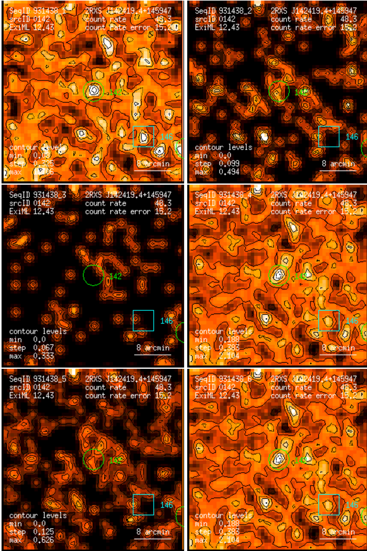
Figure 142: RASS 931438: detection 0142: band rate images, Gaussian filter: (1) PSPC channels 11 – 41, (2) 52 – 90, (3) 91 – 201, (4) 11 – 235, (5) 52 – 201, (6) 11 – 201. Broad band rates in counts/ks. Band rate contour levels in counts/ks/arcmin 2 .
