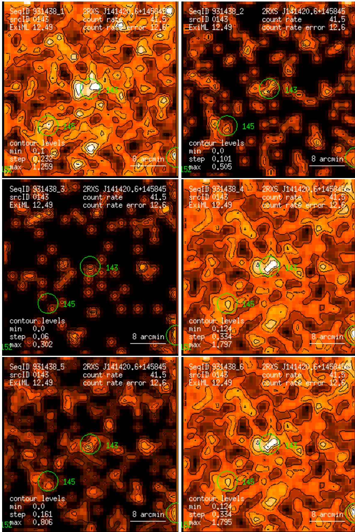
Figure 143: RASS 931438: detection 0143: band rate images, Gaussian filter: (1) PSPC channels 11 – 41, (2) 52 – 90, (3) 91 – 201, (4) 11 – 235, (5) 52 – 201, (6) 11 – 201. Broad band rates in counts/ks. Band rate contour levels in counts/ks/arcmin 2 .
