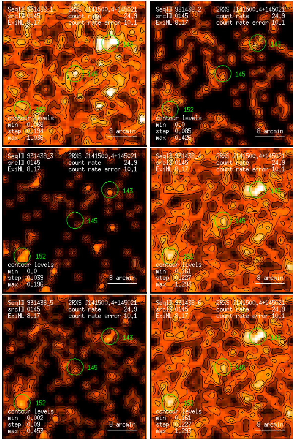
Figure 145: RASS 931438: detection 0145: band rate images, Gaussian filter: (1) PSPC channels 11 – 41, (2) 52 – 90, (3) 91 – 201, (4) 11 – 235, (5) 52 – 201, (6) 11 – 201. Broad band rates in counts/ks. Band rate contour levels in counts/ks/arcmin 2 .
